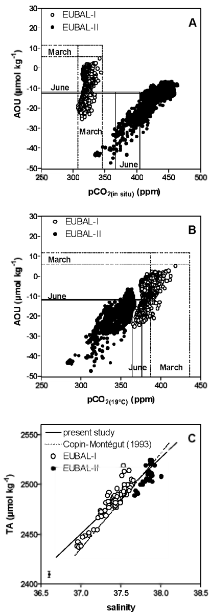
Fig. 9. (A) Apparent oxygen utilisation (AOU) versus pCO 2(in situ) and (B) AOU versus pCO 2 normalized to a constant temperature (pCO 2(19°C) ) in surface waters from all the surveys during EUBAL-I and II cruises. The range of variation of AOU and pCO 2(19°C) at the Dyfamed station for the March 1998–1999 and June 1998–1999 periods (Copin-Montégut and Bégovic, 2002; Bégovic and Copin-Montégut, 2002) are indicated by the horizontal and vertical lines. (C) Total alkalinity (TA) versus salinity in surface waters during the EUBAL-I and II cruises. Dotted line corresponds to the regression function reported by Copin-Montégut (1993) for the Alboran Sea ( TA = -1072 (\pm 16) + 94.85 (\pm 0.4) \times \text{salinity} ) and the solid line corresponds to the regression function based on the EUBAL-I and II cruises ( TA = -346 (\pm 7) + 75.6 (\pm 3) \times \text{salinity} ; r^2 = 0.869 ; n = 119 ; p < 0.0001 ). The error bar on the lower left corner of the plot corresponds to the estimated accuracy on TA measurements.
