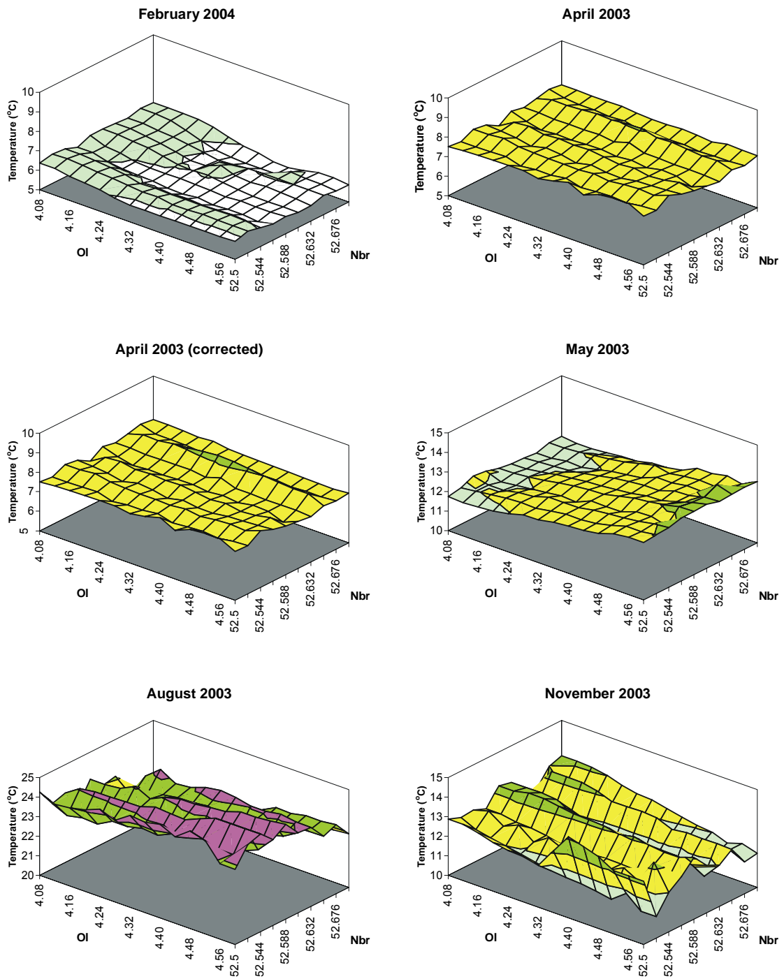
Figure 8. Three-dimensional plots of temperature against geographical coordinates.
