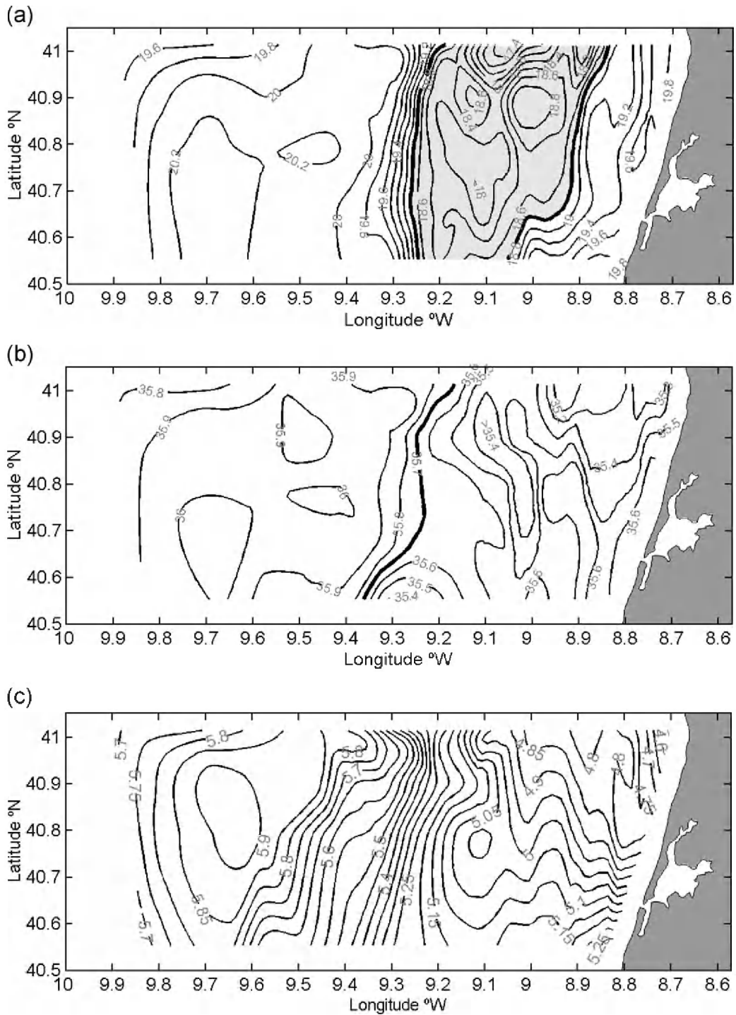
Fig. 5. Surface distributions of: (a) temperature (°C). The zone with colder waters (<18.8°C) is represented in shaded areas; (b) salinity (psu); and (c) surface geopotential anomaly (m 2 s -2 ) relative to 480 dbar.
