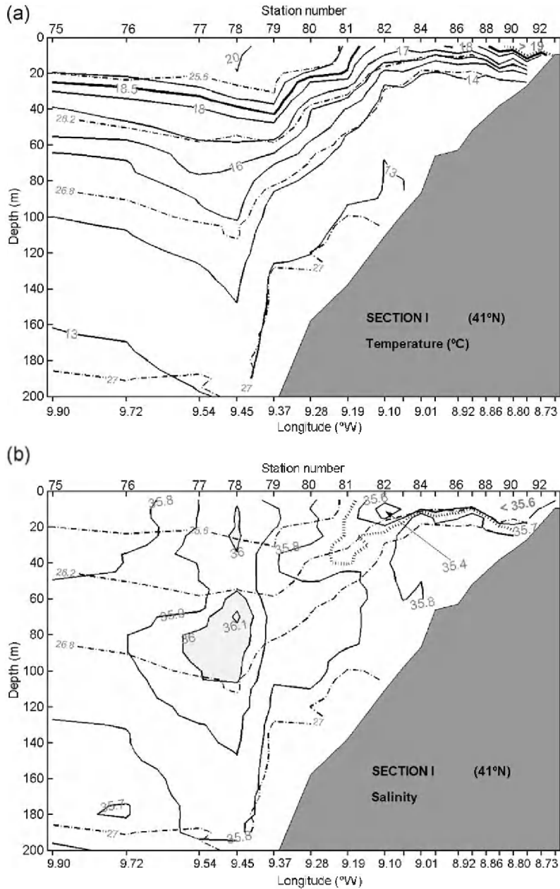
Fig. 6. Vertical fields in section I: (a) temperature ( ^{\circ}\text{C} ) (solid lines); (b) salinity (psu) (solid lines) and (c) geostrophic velocities ( \text{m s}^{-1} ) referenced to 480 dbar (positive values correspond to northward velocity are shaded). Dashed–dotted lines on (a) and (b) represent \sigma_t . Thick dotted line represents the Western Iberian Buoyant Plume (WIBP).
