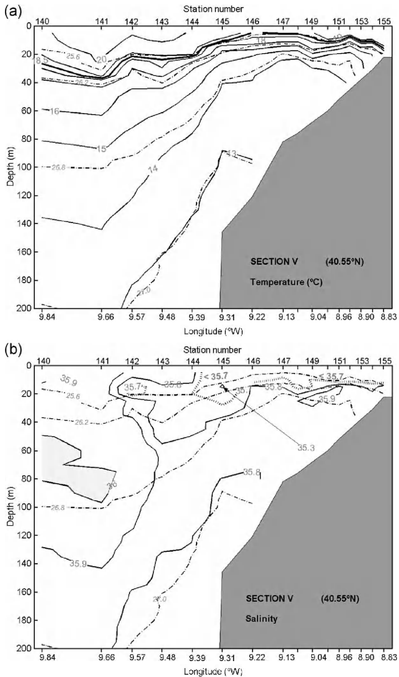
Fig. 7. Vertical fields in section V: (a) temperature ( ^{\circ}\text{C} ) (solid lines); (b) salinity (psu) (solid lines) and (c) geostrophic velocities ( \text{m s}^{-1} ) referenced to 480 dbar (positive values correspond to northward velocity are shaded). Dashed–dotted lines on (a) and (b) represent \sigma_t . Thick dotted line represents the Western Iberian Buoyant Plume (WIBP).
