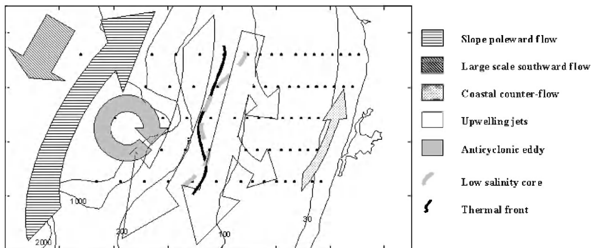
Fig. 8. Conceptual scheme of the circulation on the surveyed area.
