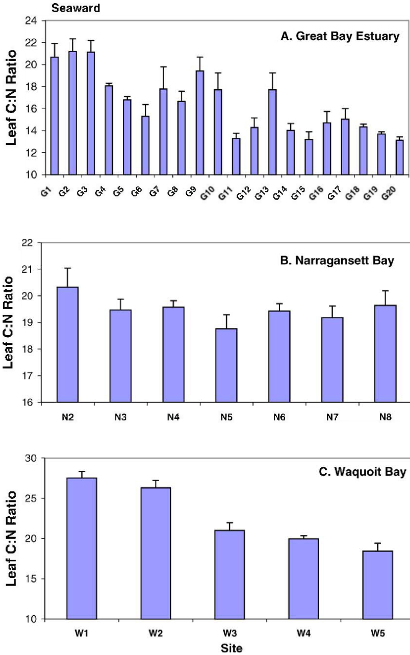
Fig. 3. Ratios of carbon to nitrogen content of eelgrass leaves along estuarine gradients in Great Bay Estuary (A), Narragansett Bay (B), and Waquoit Bay (C).
