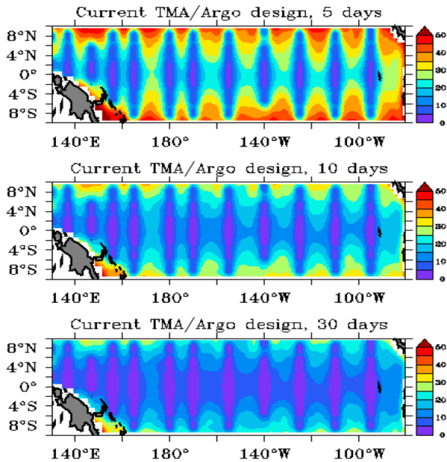
Figure 5-1: A calculation of the error as a percentage of the temperature variance signal at \sigma=25 depth that can be recovered using current TMA and Argo sampling designs. The covariance function is the one used in Gasparin et al. (2015), with percentage errors estimated at different timescales: 5 days (upper), 10 days (middle) and 30 days (lower). Red denotes large errors and poor signal recovery. Courtesy of Florent Gasparin.
