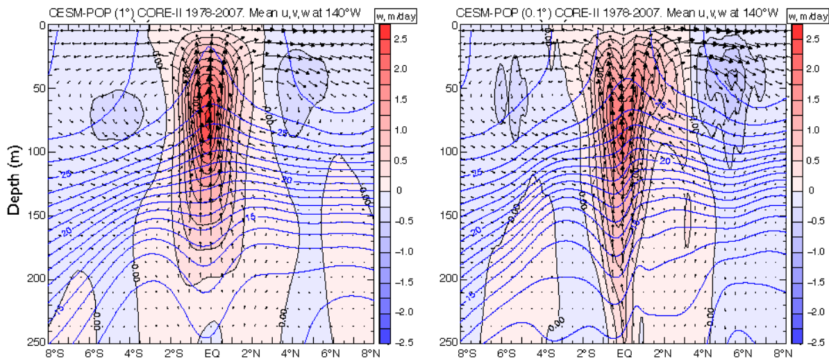
Figure 6-2. Circulation in the meridional plane at 140°W in coarse (1° in longitude, left) and fine resolution (0.1°, right) versions of the Community Earth System Model (CESM) OGCM forced by identical Common Ocean Reference Experiment fluxes (Tseng et al., 2016). Vertical velocity is shaded in units of meters/day. Vectors represent 10-day displacements. The parameterization of small-scale vertical mixing in the low- and high-resolution models is identical.
