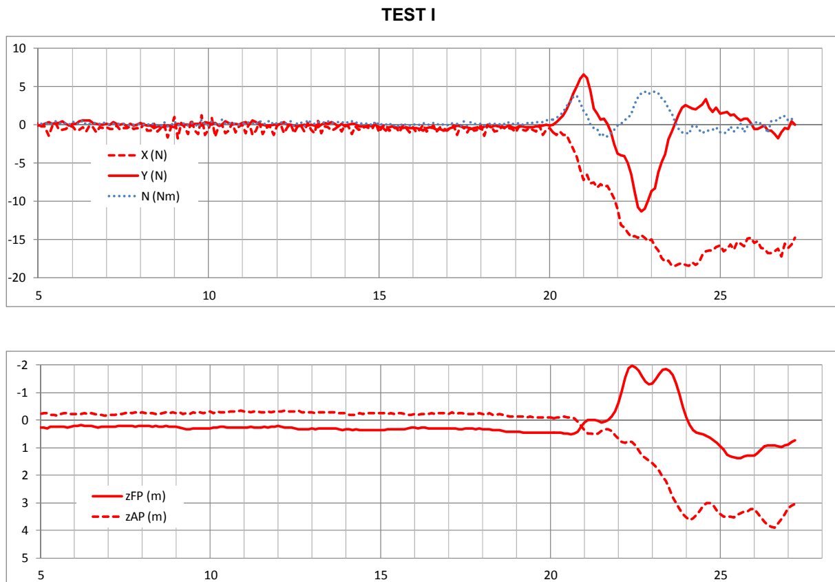
Figure 17. Benchmark test I
