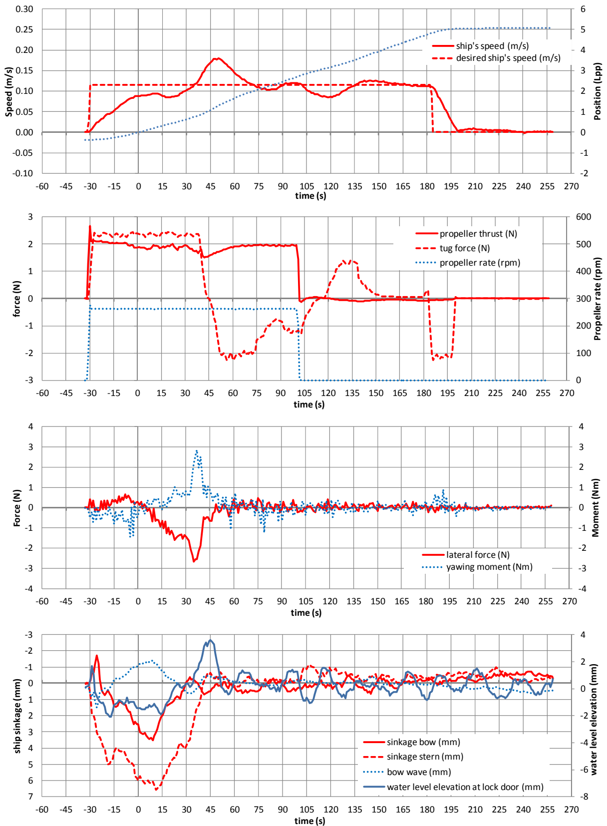
Figure 8. Benchmark test C (029).
