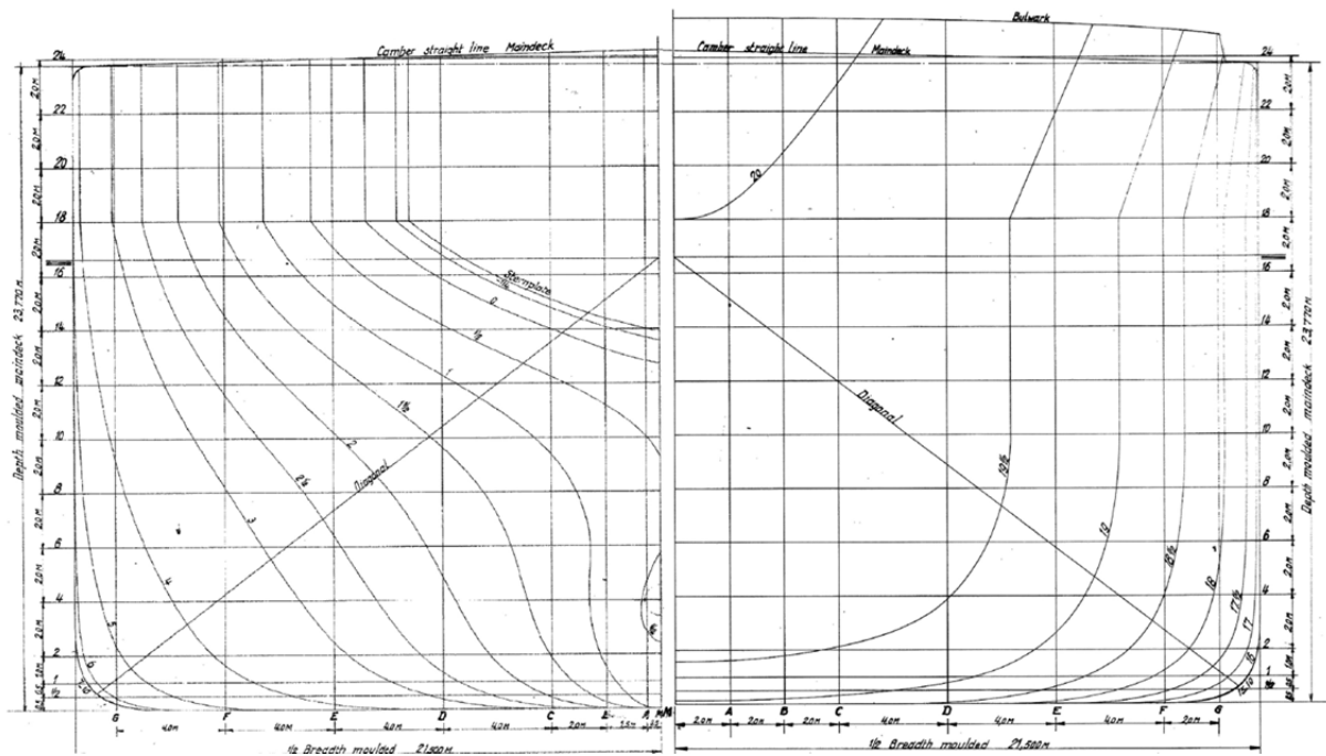
Figure 14. 1/75 scale model of bulk carrier used during captive benchmark tests: body plan
