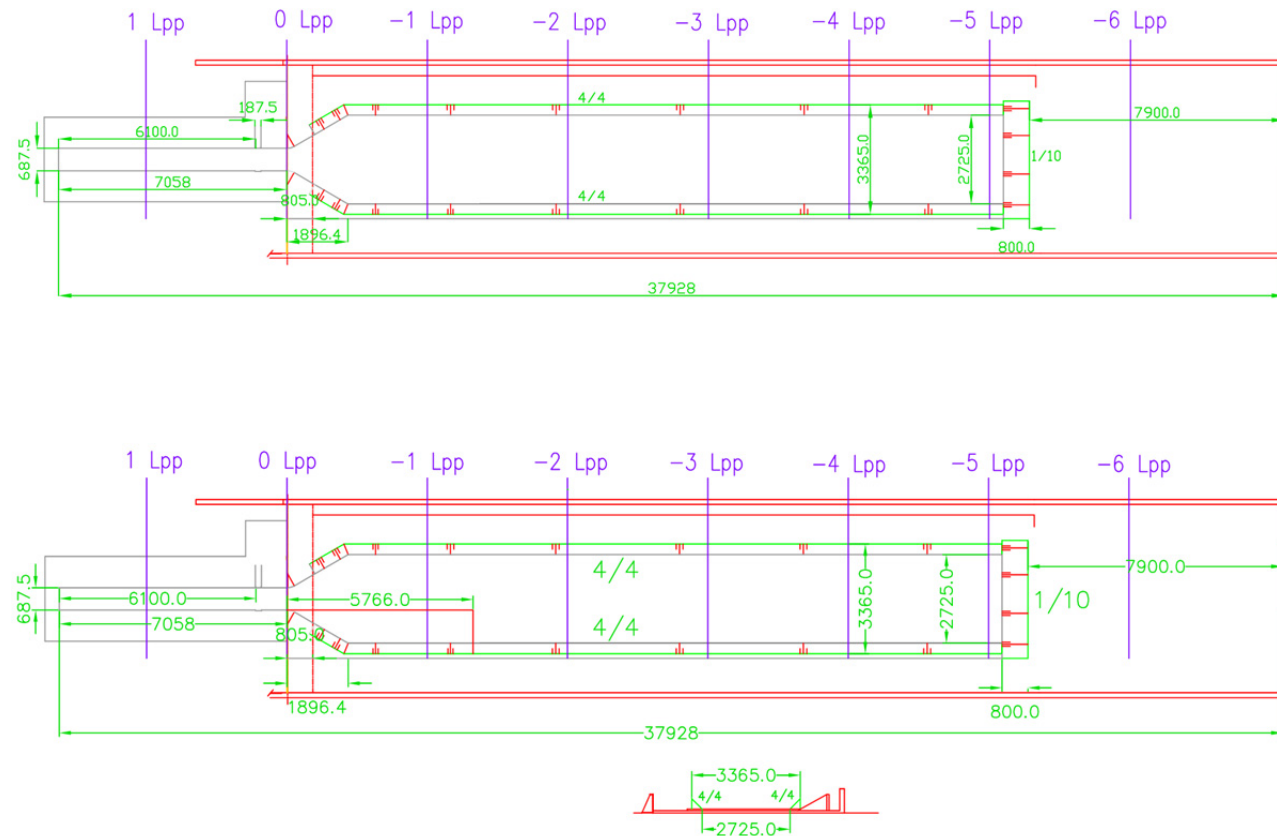
Figure 3. Different approach wall configurations on the Pacific entrance: No approach wall (top) – Closed approach wall (bottom).
