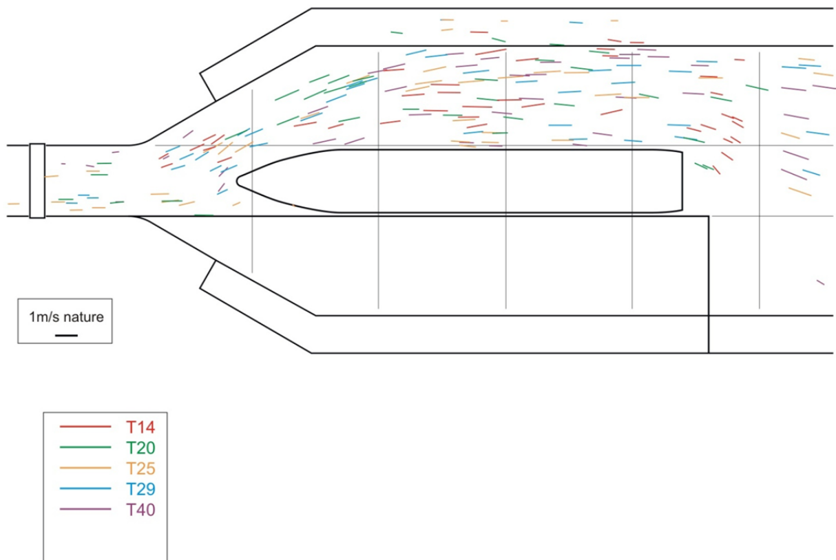
Figure 12. Benchmark test F: surface flow at discrete time steps ( T_m denotes the situation m minutes full scale after the start of the test; m has to be multiplied by 6.7 to obtain the model time in seconds).
