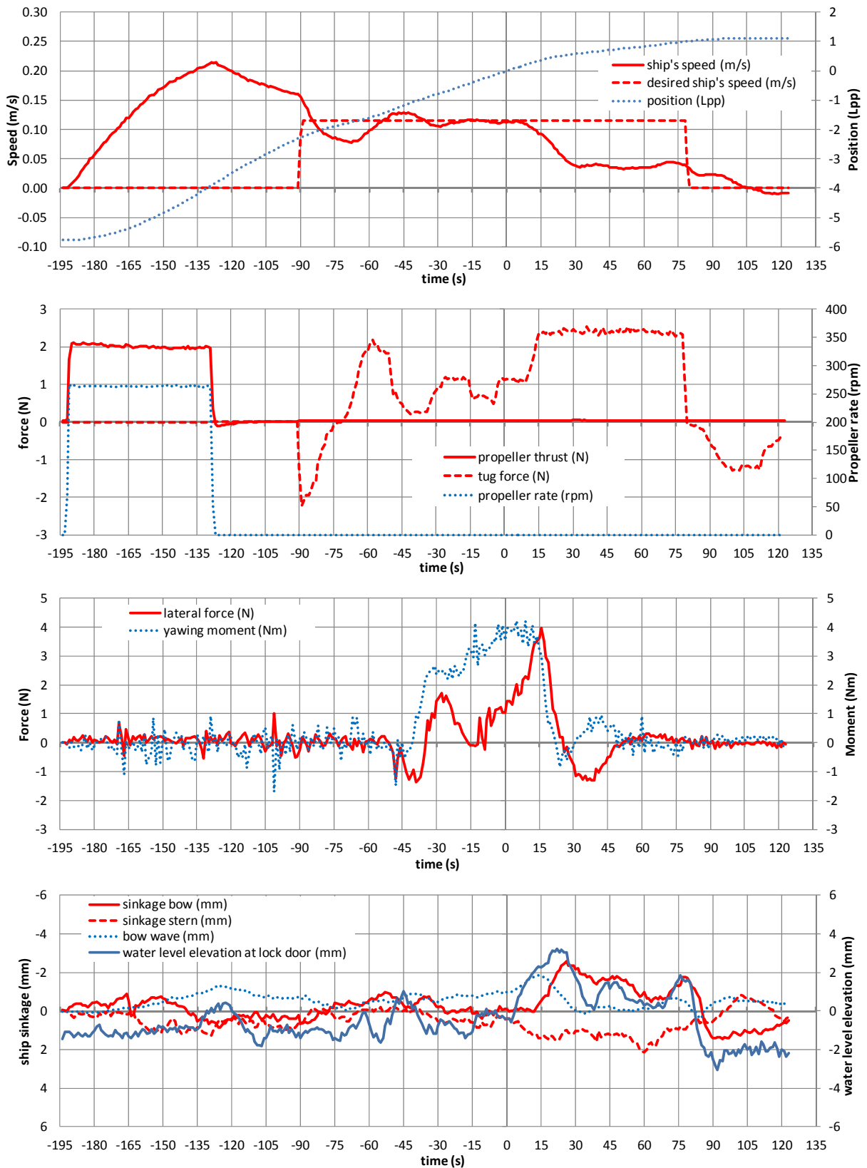
Figure 7. Benchmark test B (121).
