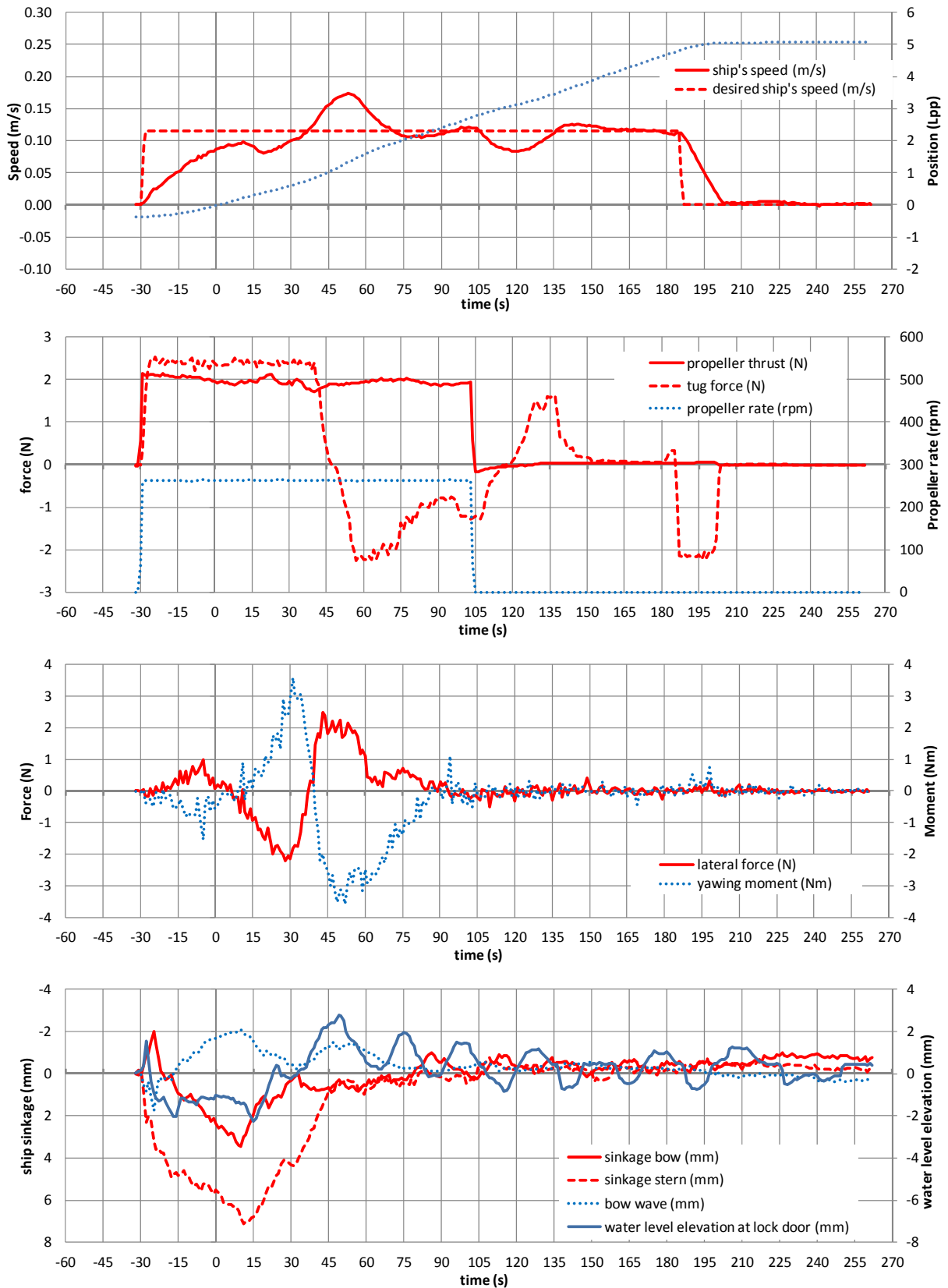
Figure 9. Benchmark test D (117).
