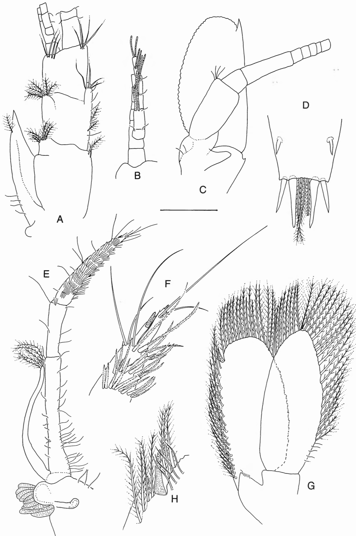
Figure 2. Salmones colinorum sp. nov. ovig. paratype pocl 3.35 mm (OUMNH 2002-24-45). A: antennular peduncle; B: detail of lateral antennular flagellum; C: scaphocerite and antennal peduncle; D: tip of telson; E: third maxilliped; F: tip of same; G: uropod; H: lateral spine of exopod. Scale bar indicates 0.65 mm (A, C, E, G), 0.50 mm (B, D) or 0.20 mm (F, H).
