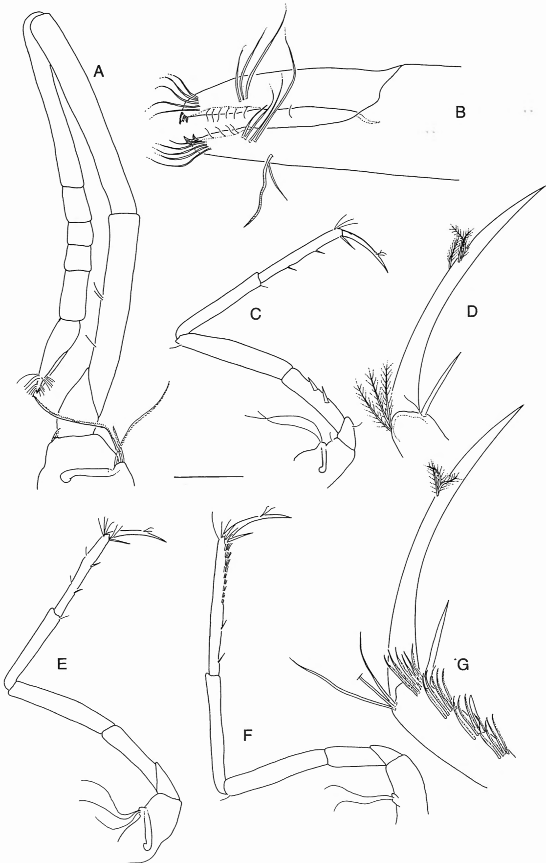
Figure 4. Salmoneus colinorum sp. nov, ovigerous paratype pool 3.35 mm (OUMH 2002-24-45). A: second pereiopod; B: same, fingers; C: third pereiopod; D: same, distal part; E: fourth pereiopod; F: fifth pereiopod; G: same, distal part. Scale bar indicates 1 mm (C, E, F), 0.4 mm (A) or 0.2 mm (B, D, G)
