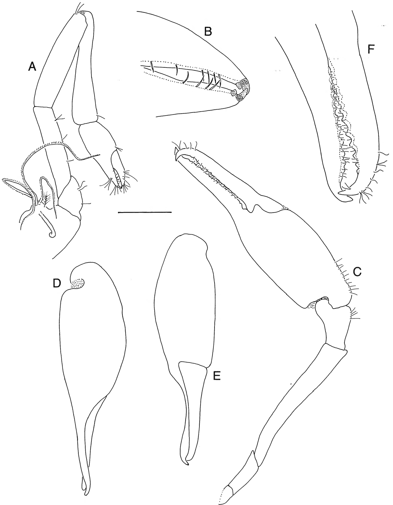
Figure 3. Salmoneus colinorum sp. nov, ovigerous paratype pochl 3.35 mm (OUMNH 2002-24-45). A: minor cheliped; B: same, finger tips; C: major cheliped; D: same, palm, dorsal view; E: same, palm, ventral view; F: same, finger tips. Scale bar indicates 1 mm (C, D-E), 0.5 mm (A, F) or 0.1 mm (B).
