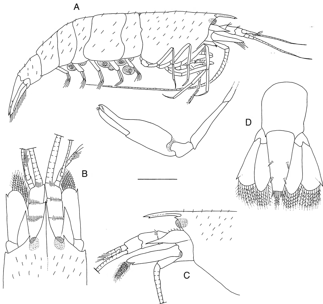
Figure 1. Salmeoneus colinorum sp. nov, holotype (OUMNH 2002-24-44) (A, B, C), ovig. paratype pochl 3.00 mm (KBIN IG 30230) (D). A: lateral view (major cheliped detached); B: frontal region, dorsal view; C: same, lateral view; D: caudal fan. Scale bar indicates 2 mm (A) or 1 mm (B-D)
