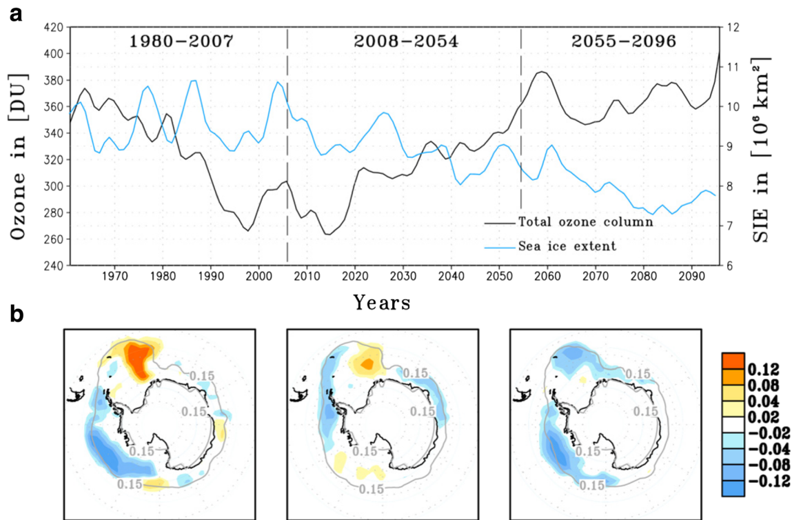
Fig. 4 a Evolution of the Antarctic total ozone column (in Dobson Unit, DU, 60^\circ \text{ S}–90^\circ \text{ S} mean, black ) in October and Antarctic sea ice extent (SIE, in \text{km}^2 , blue ) in December between 1960 and 2100, simulated with the EMAC chemistry-climate model, assuming the RCP6.0 greenhouse gas scenario and the WMO-A1 scenario for ozone depleting substances.
