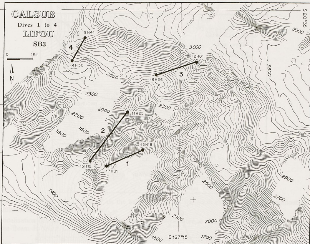
FIG. 7. — Location of dives 1 to 4 off the North of Lifou island. Map without extrapolation, from multibeam sounder of R/V J. Charcot .
