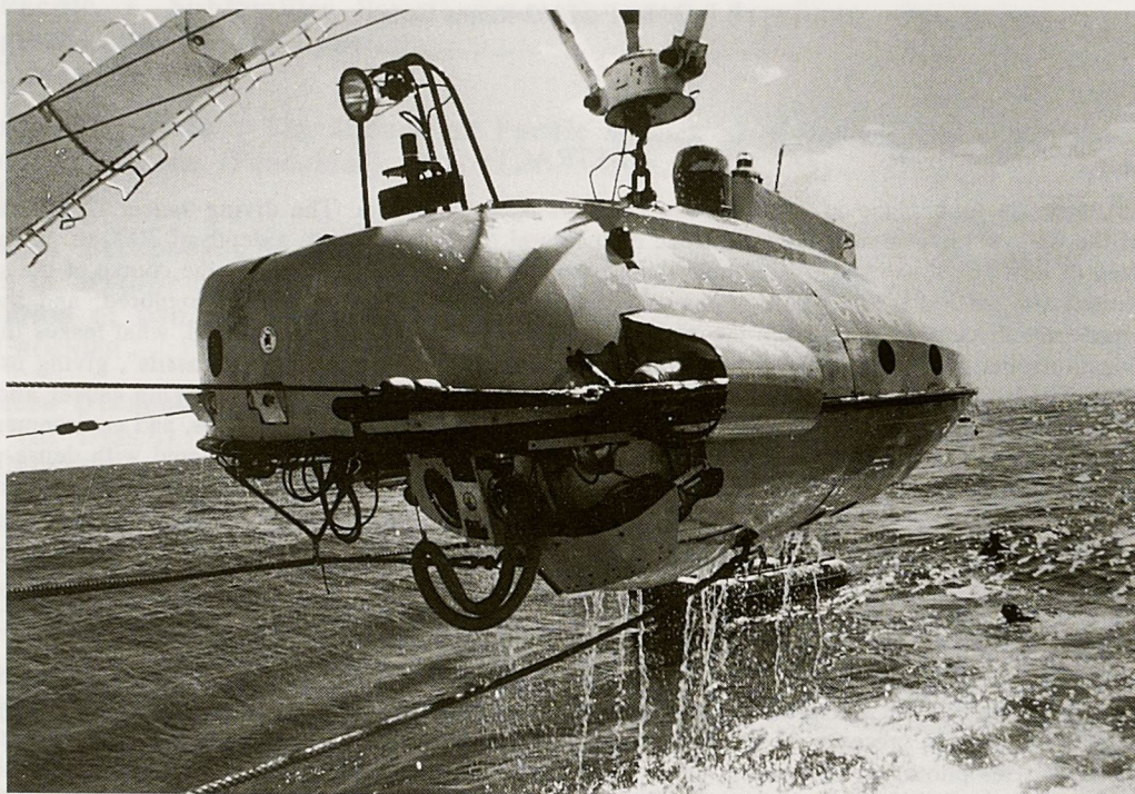
FIG. 1. — Recovery of SP 3000 Cyana at the end of a dive during the CALSUB cruise.
