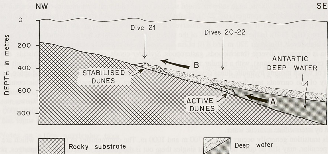
FIG. 15. — Axial profile of the epibathyal gulley between the Isle of Pines and the Great Southern Reef.
