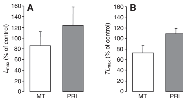
Fig. 8. Effects of the guanylyl cyclase inhibitor ODQ ( 10^{-5} mol l ^{-1} ) on (A) L_{\max} and (B) TL_{\max} of the hormonally ( 10^{-6} mol l ^{-1} ) induced luminescence from E. spinax photophores. ODQ had no effect on this light emission. Values are expressed as a percentage of values obtained in control photophore preparations, i.e. VSP stimulated with MT or PRL alone. N=8 for each experiment.
