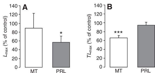
Fig. 5. Effects of the NO donor hydroxylamine ( 10^{-3} mol l ^{-1} ) on (A) L_{\max} and (B) TL_{\max} of hormonally ( 10^{-6} mol l ^{-1} ) induced luminescence from E. spinax photophores. Values are expressed as a percentage of values obtained in control photophore preparations, i.e. VSP stimulated with MT or PRL alone. N=8 for each experiment. Asterisks indicate significant differences between control and treated VSP: * P<0.05 , *** P<0.001 .
