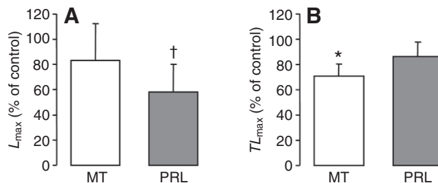
Fig. 7. Effects of the cGMP analogue 8Br-cGMP ( 10^{-4} mol l ^{-1} ) on (A) L_{\max} and (B) TL_{\max} of the hormonally ( 10^{-6} mol l ^{-1} ) induced luminescence from E. spinax photophores. Values are expressed as a percentage of values obtained in control photophore preparations, i.e. VSP stimulated with MT or PRL alone. N=8 for each experiment. Asterisks indicate significant differences between control and treated VSP: * P<0.05 , † P=0.06 .
