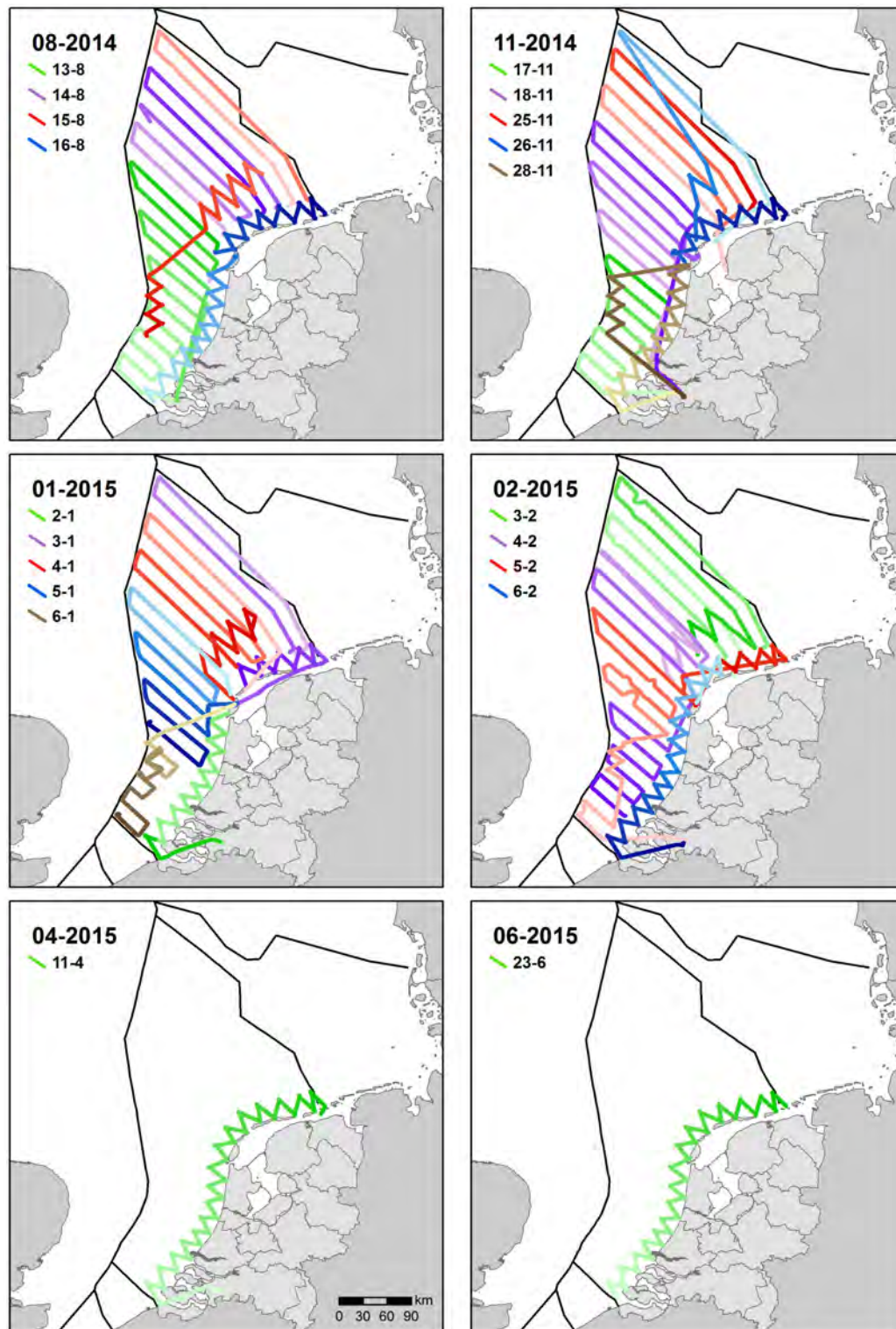
Figure II.2 Datumspreiding en gebiedsdekking van de monitoringsvluchten in 2014-2015 op het NCP. Kleursterkte is een indicatie van vliegrichting vliedend van mild naar intens. Survey timing and spatial coverage of aerial surveys during the 2014-2015 monitoring on the DCS. To provide an indication of the order that transects were flown, the colour of each day's transects fades throughout the day.
