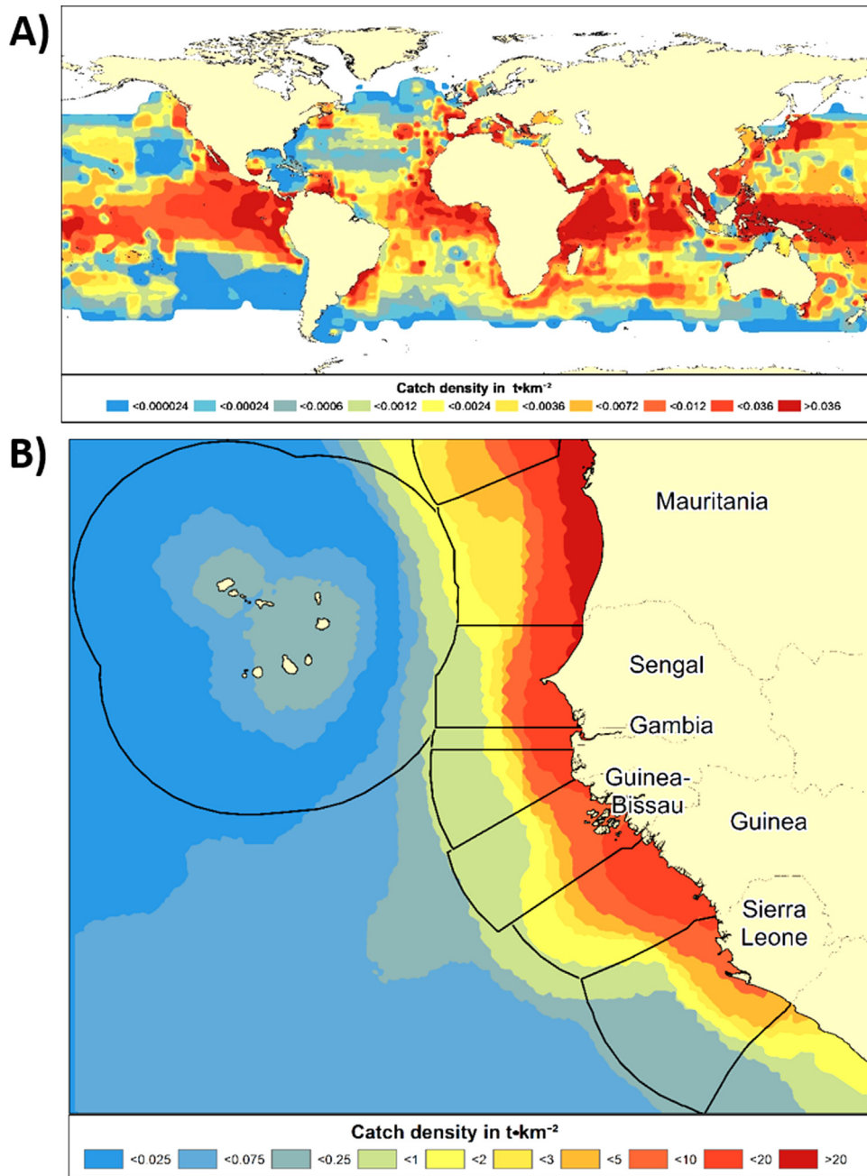
Fig. 5. The global databases and spatial allocation procedure of the Sea Around Us allows the mapping of catches in space and time, e.g., of (A) the global average annual catches ( \text{t km}^{-2} ) of large pelagic species (mainly tuna and billfishes) for 2000–2010 as derived from various sources; and (B) the average catches by all fishing countries in and around the EEZs of Senegal and The Gambia and neighboring areas for 2000–2010 [24,35].
