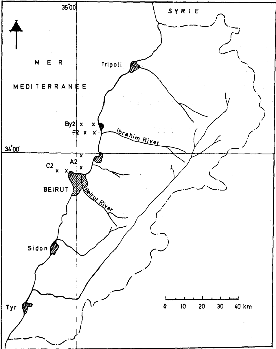
Fig. 1 — Location of plankton transects and stations along the coast of Lebanon.
