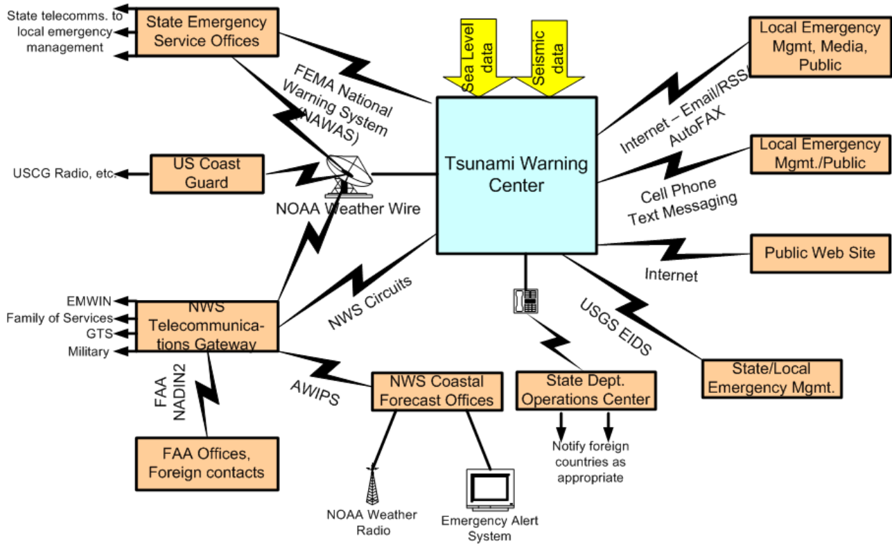
Figure 5.2 WC/ATWC message dissemination
