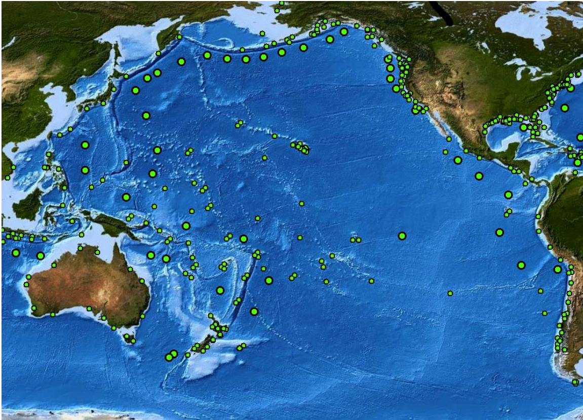
Figure 3.4 Coastal sea level stations (small dots) and deep ocean sea level stations (larger dots) in the Pacific that are monitored by PTWC and WCATWC for the detection and measurement of tsunamis. August 2011.
