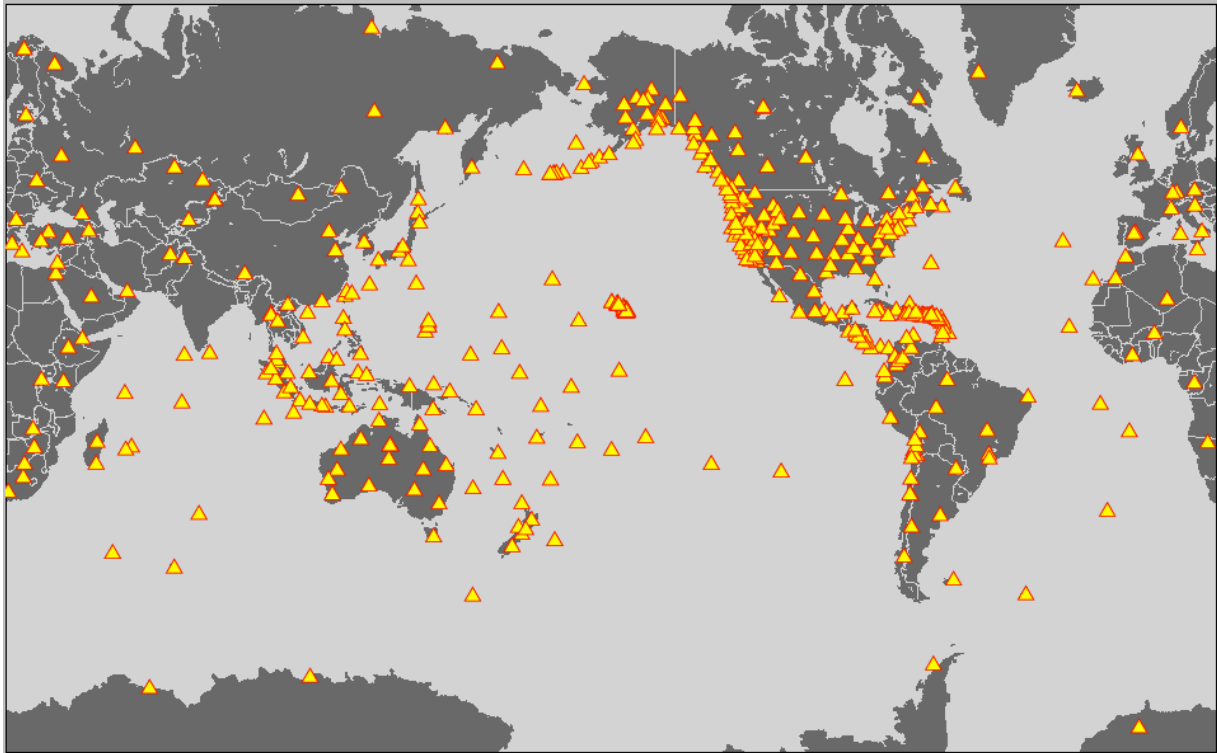
Figure 3.3 Seismic stations in the Pacific region monitored by PTWC for the detection and evaluation of large, potentially tsunamigenic earthquakes. August 2011.
