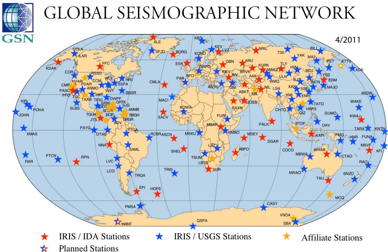
Figure 3.2 Global Seismographic Network (GSN)
