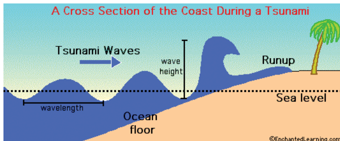
Figure 2.3 Physic characteristics of tsunami waves. ( http://trestlessurfcrowd.wordpress.com/2010/02/28/tsunami-physics-and-trestles/ )
