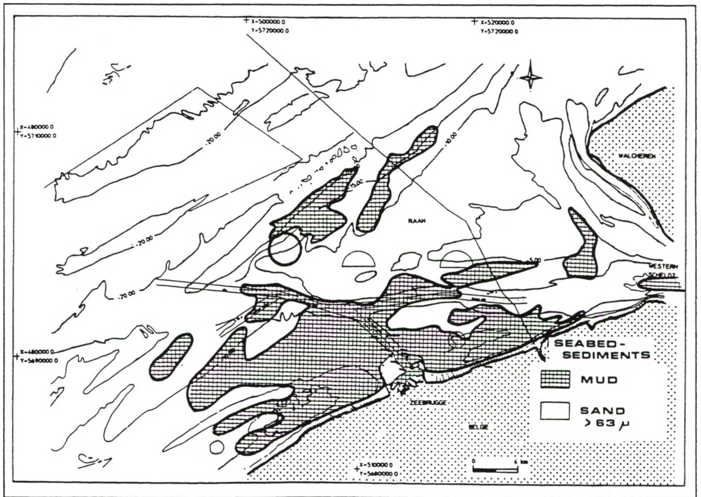
Figure 6. Lithological map of the study area indicating distribution of sand and mud sealed sediments.
