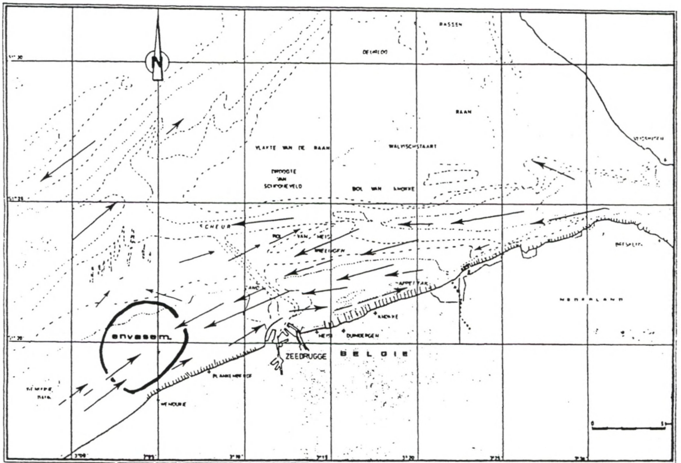
Figure 10 : Residual sediment transport directions before harbour extension (1975-1977)
