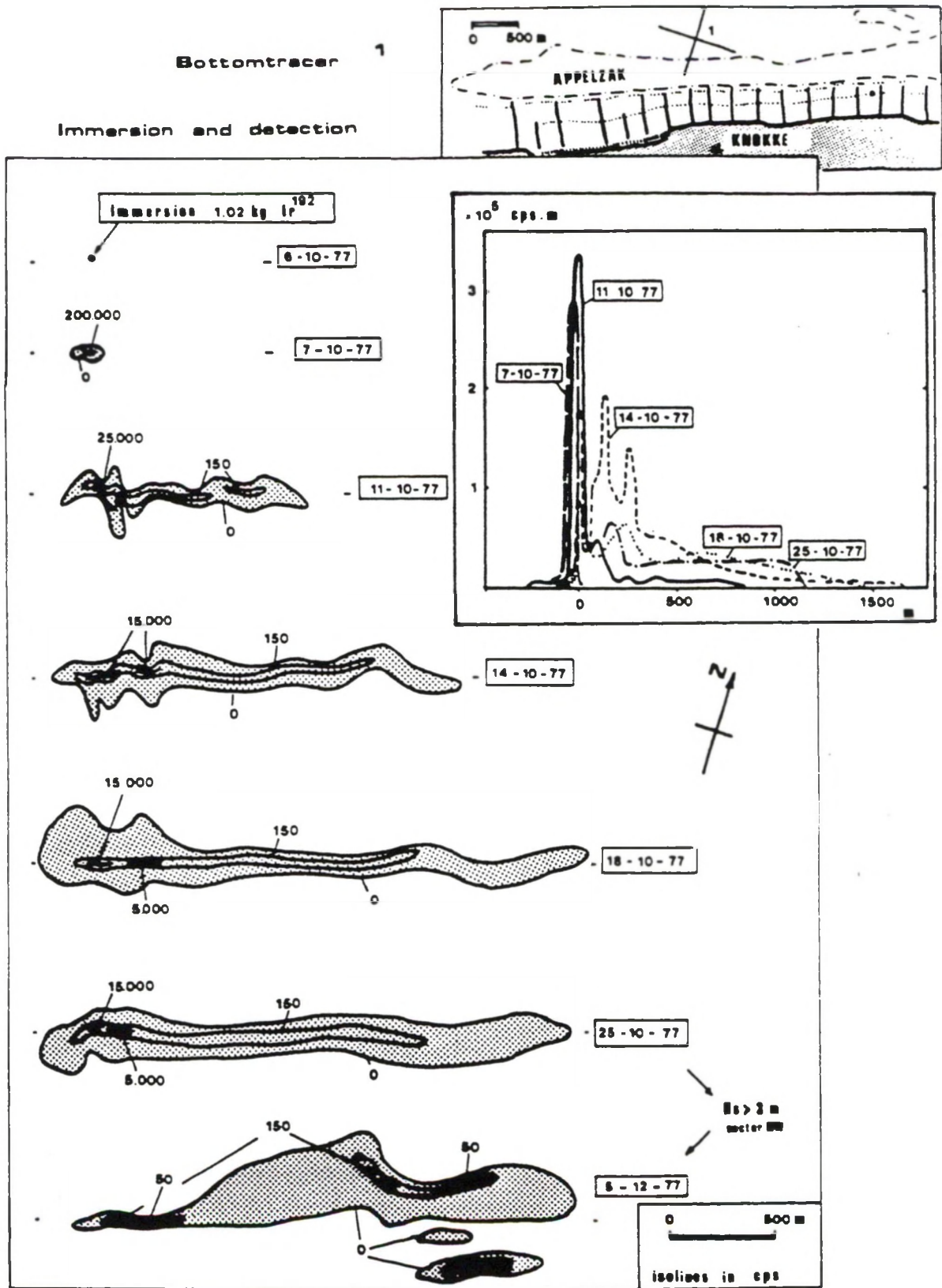
Figure 14. Bed-load transport; measurements with radioactive tracers. Example of detection results yielding residual sediment transport directions and discharges under combined tidal current and wave actions
