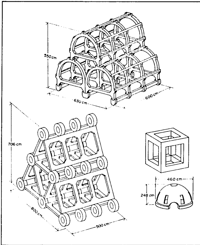
Fig. 8. Examples of Japanese chambered concrete modules used in constructing artificial reefs with large void spaces. 13,37
