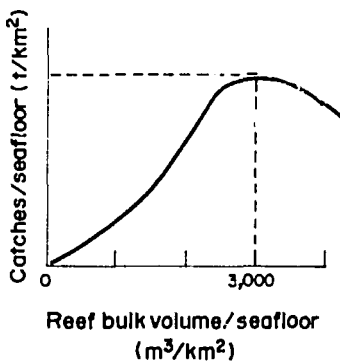
Fig. 2. Dependence of fish catches on reef density showing catches versus reef bulk volume per km 2 of sea bottom. 53
