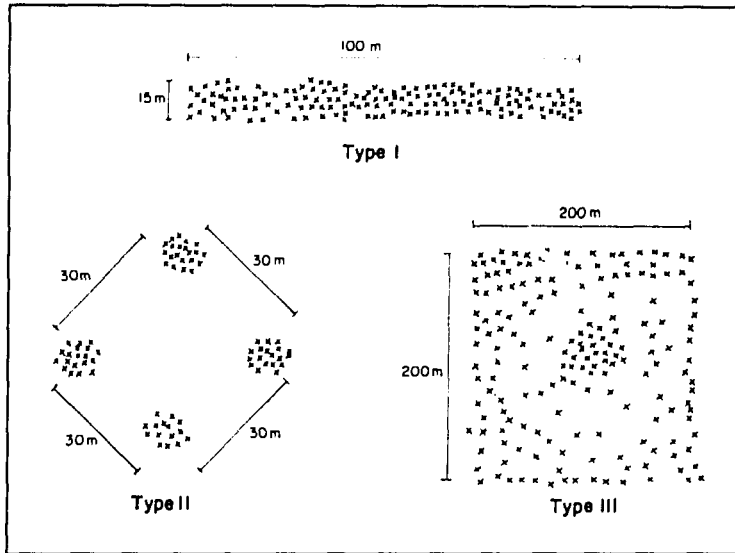
Fig. 16. Three arrangements of artificial reefs used in Thailand for distinct purposes. 50
