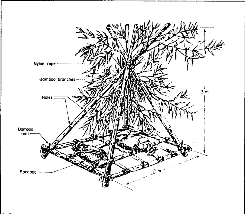
Fig. 13. A pyramid bamboo module used in the Philippines. 34
