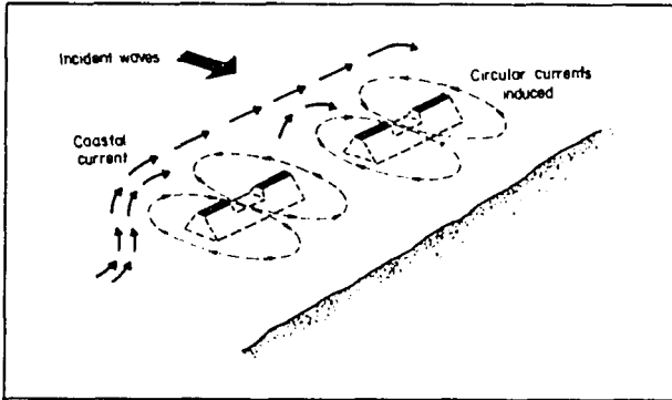
Fig. 17. Creation of circular currents with submerged breakwaters to enhance recruitment of abalone larvae. 60
