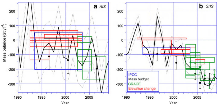
Fig. 3 Recent mass balance estimates ( \text{Gt year}^{-1} ) for the AIS (left) and the GrIS (right), based on altimetry (red), GRACE (green) and the mass budget method (black). MB data from Fig. 2 are plotted as black dashed lines with uncertainty margins. Data sources AIS (left): Wingham et al. (1998); Rignot and Thomas (2002); Davis et al. (2005); Zwally et al. (2005); Velicogna and Wahr (2006b); Ramillien et al. (2006); Wingham et al. (2006); Chen et al. (2006b); Bindoff et al. (2007); Helsen et al. (2008); Rignot et al. (2008b); Chen et al. (2009); Data sources GrIS (right): Krabill et al. (2000); Krabill et al. (2004); Velicogna and Wahr (2005); Thomas et al. (2006); Rignot and Kanagaratnam (2006); Ramillien et al. (2006); Chen et al. (2006a); Luthke et al. (2006); Bindoff et al. (2007); Wouters et al. (2008); Rignot et al. (2008a); Cazenave et al. (2009); Velicogna (2009); Schrama and Wouters (2011)
