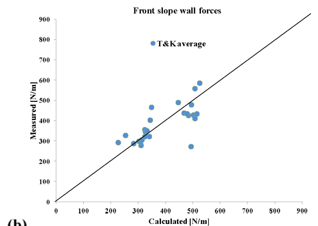
Figure 4. Measured versus calculated forces on the front sloping wall. (a) T&K and T&K(impulsive) design formula. (b) T&K average of impulse and no impulsive Goda formula.
