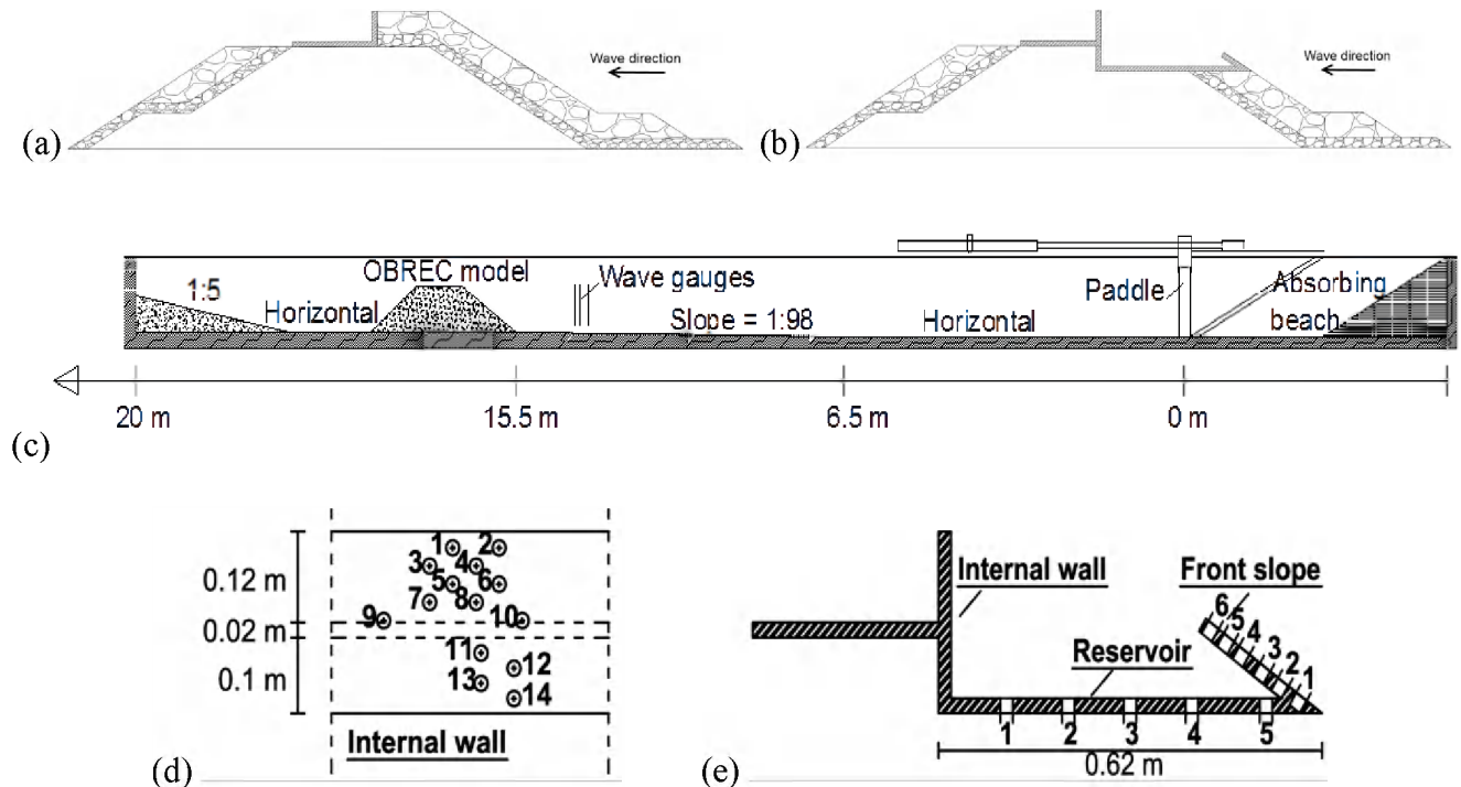
Figure 1. Model tested at Aalborg University. (a) Cross-section of traditional rubble mound breakwater. (b) Cross-section of Overtopping BReakwater for Energy Conversion ( OBREC ). (c) Layout of model test in 2D wave flume. (d) Frontal view of the internal reservoir wall and pressure transducers location. (e) Cross-section of the internal reservoir wall, front sloping wall and reservoir bottom and pressure transducers location.
