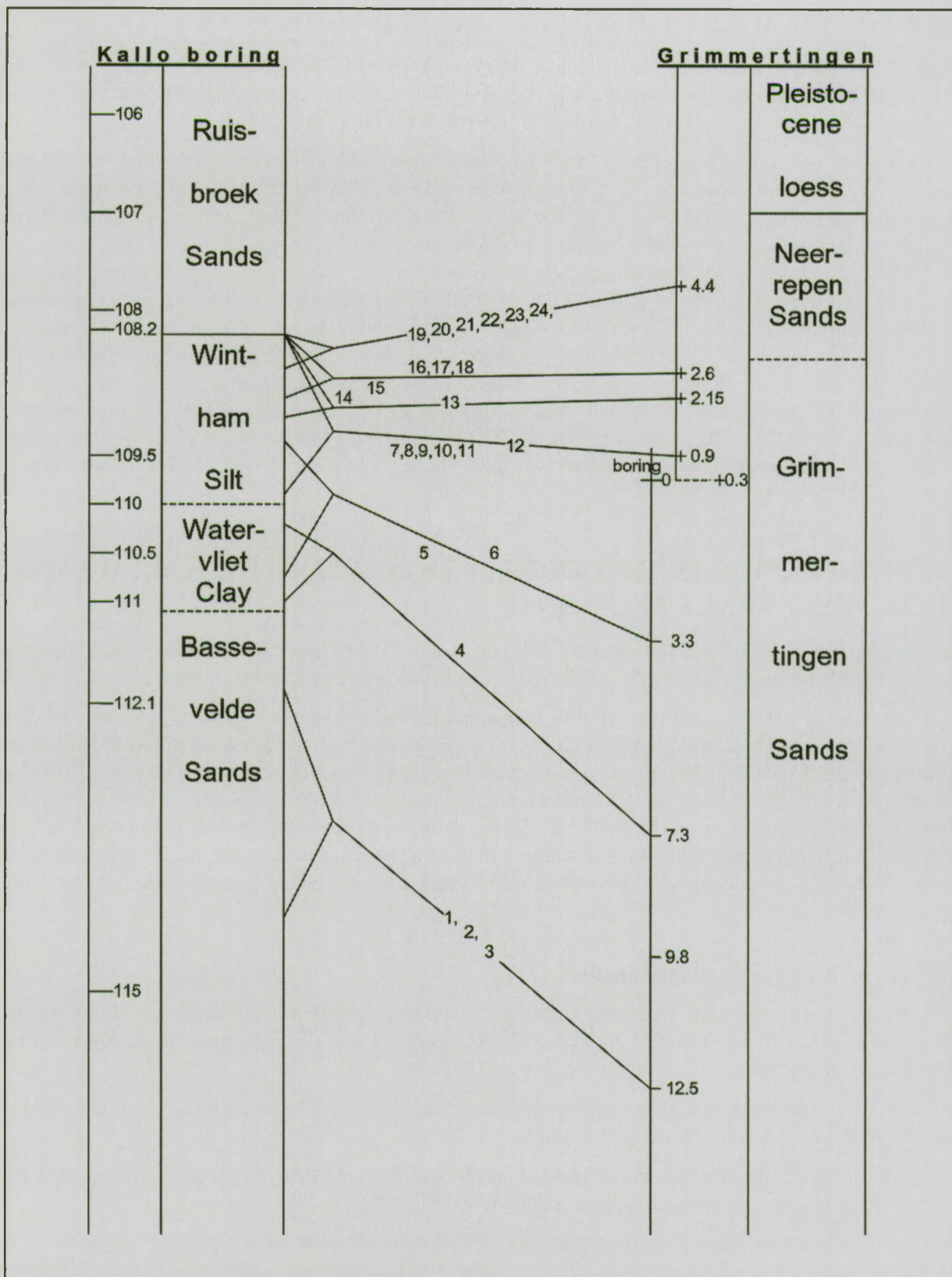
Figure 3: Biostratigraphic correlations between the Grimmertingen section and the Kallu reference section. First appearances in the Grimmertingen section are marked by numbers just above the lines tracing the correlations; last appearances by numbers just below these lines. Numbers written on the lines represent species which may eventually be found below the corresponding level (1 to 3) or above (19-24), or which have been observed at one level only (12 and 13).
