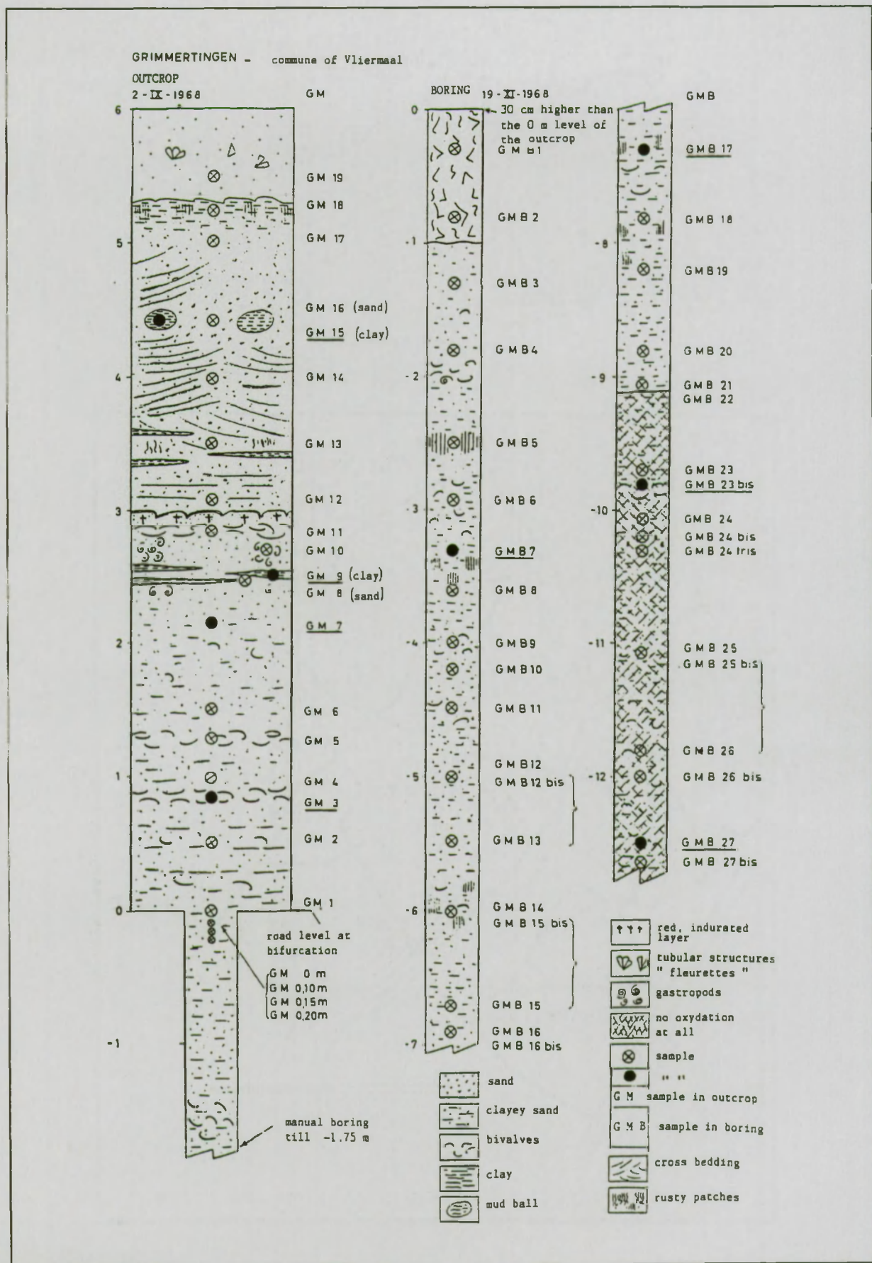
Figure 2: Lithology of the Grimmertingen section and position of the samples.
