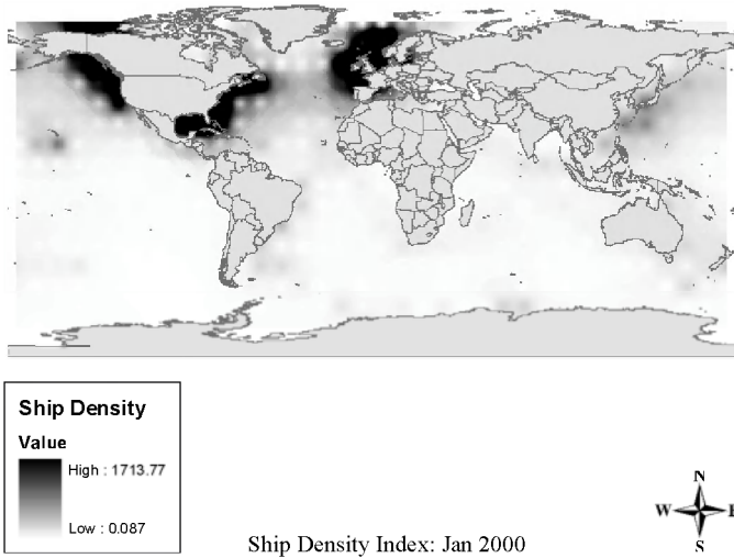
Figure 2. Ship Density Index: the distribution is representing the month of January 2000.
