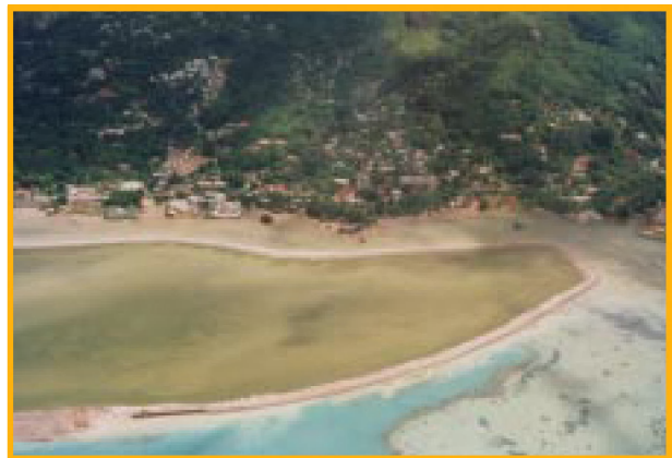
Lagoons and reef flats are destroyed in land reclamation schemes, particularly on islands where land is in short supply.
