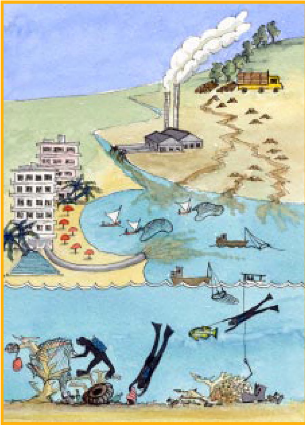
The range of threats to coral reefs from human activities.
