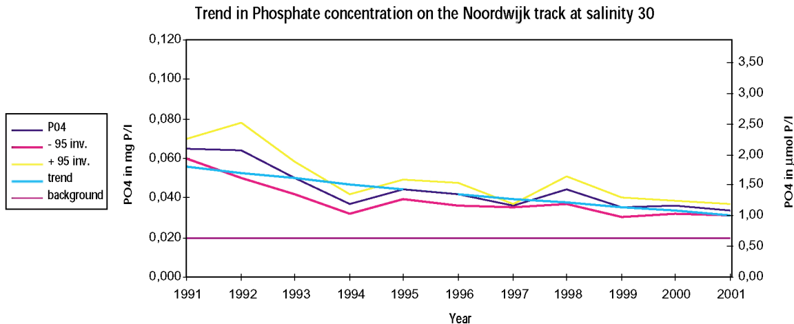
Fig. 2 shows the reduction in P-inputs, as a decline in the ortho-P- concentration on the Noordwijk track.
