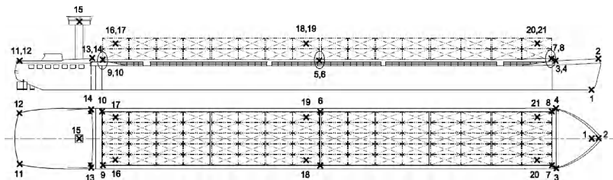
Figure 4b. Critical points to be considered in a risk analysis: container carrier.
