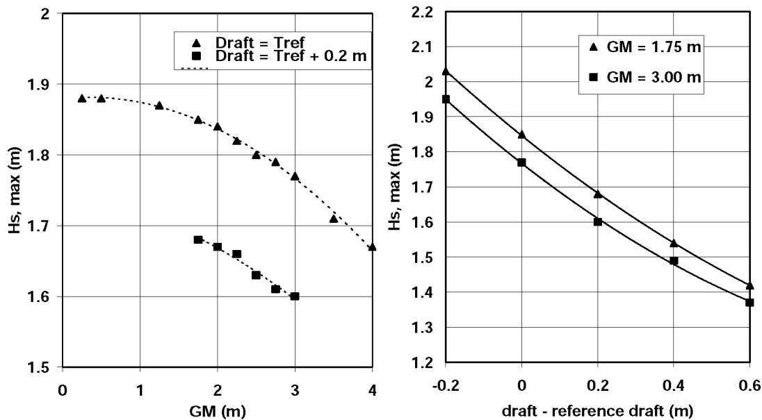
Figure 8. Estuary container vessel: maximum allowable significant wave height as a function of draft and metacentric height ( GM ).
