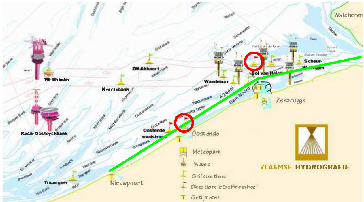
Figure 5. Measuring Network Flemish Banks (Meetnet Vlaamse Banken). Trajectories (green lines) for estuary traffic Western Scheldt – Zeebrugge – Nieuwpoort and locations of directional wave buoys (red circles) Bol van Heist and Oostende. Source: adapted from Vlaamse Hydrografie.
