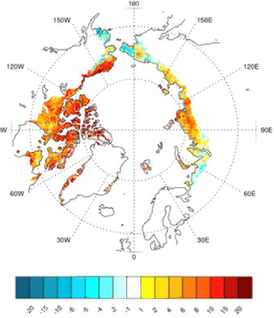
C Maximum NDVI (MaxNDVI) (percentage change, 1982-2008)
