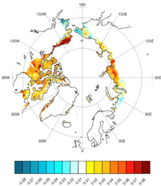
Figure V1. Magnitude (left) and percentage (right) change of maximum NDVI (MaxNDVI) from 1982 to 2008 for the circumpolar arctic tundra region. Colors show changes only within the area north of the Arctic tree line. Color scales are not linear (Bhatt et al., 2010).
