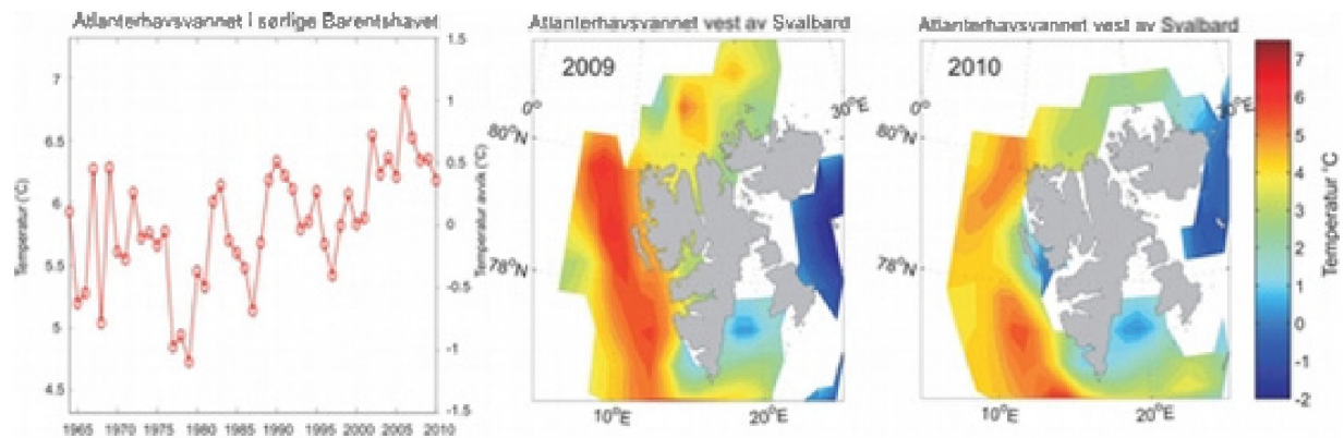
Figure BA1. The left figure shows the temperature in the Atlantic water flowing into the Barents Sea in the south. Vertical axis on the left side of the figure shows the temperature, while the axis on the right side of the figure shows the temperature deviation from the mean of the 30-year period 1977-2006. The two figures on the right show temperatures at 100 meters depth, measured in 2009 and 2010.
