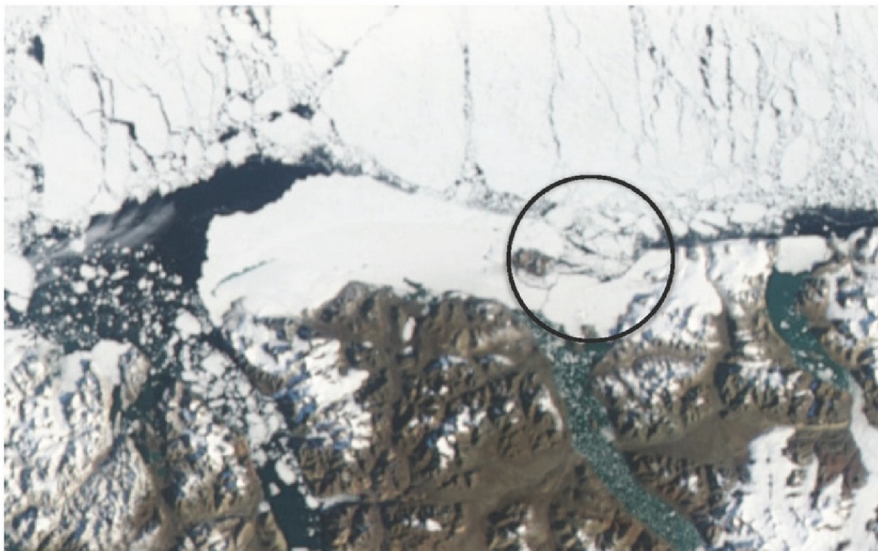
Figure G3. MODIS image from 18 August 2010 showing the breakup of the Ward Hunt Ice Shelf, Ellesmere Island, in the region to the east of Ward Hunt Island (circled). Image from NASA.
