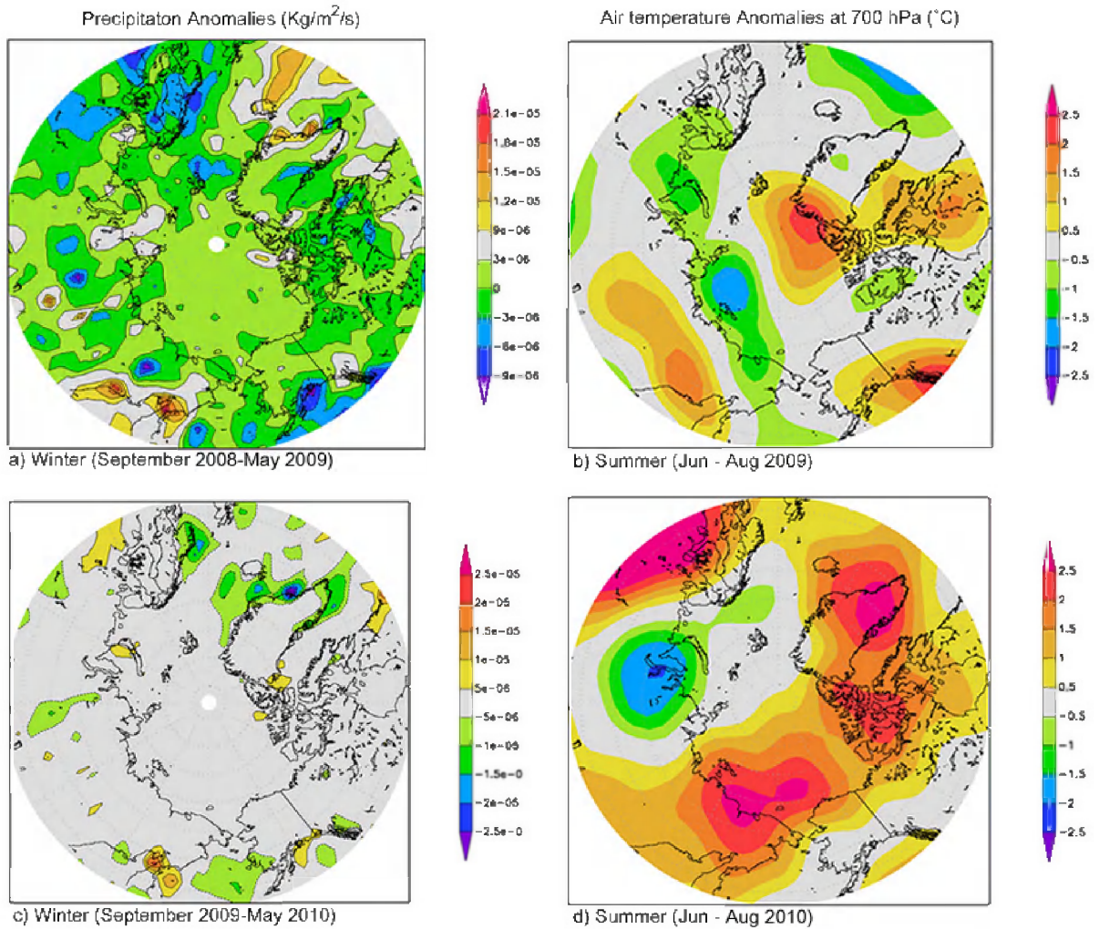
Figure G1. Anomalies (relative to 1948-2008 climatology) in: (a, top, left) winter (September 2008-May 2009) precipitation ( \text{Kg}/\text{m}^2/\text{s} ), and (b, top, right) summer (June-August) 2009 air temperature ( ^{\circ}\text{C} ) at 700 hPa, (c, bottom, left) as (a), for September 2009 - May 2010, (d, bottom, right), same as (b) for June-August 2010.
