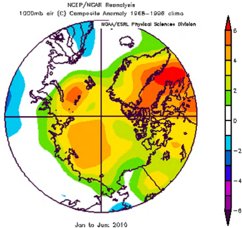
Figure A.4. Air temperature for the first half of 2010 showing anomalies of over 4°C over northeastern Canada.
