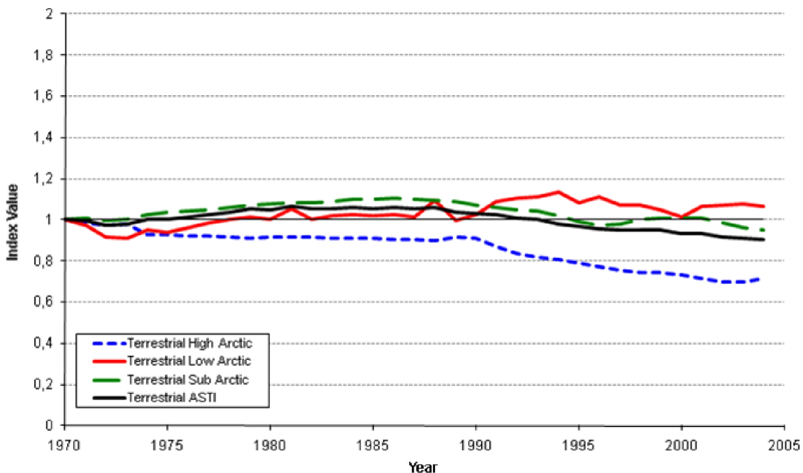
Figure W2. Index of terrestrial species disaggregated by Arctic boundary for the period 1970-2004. (High Arctic, n=25 species, 73 populations; Low Arctic, n=66 species, 166 populations; Sub Arctic, n=102 species, 204 populations)
