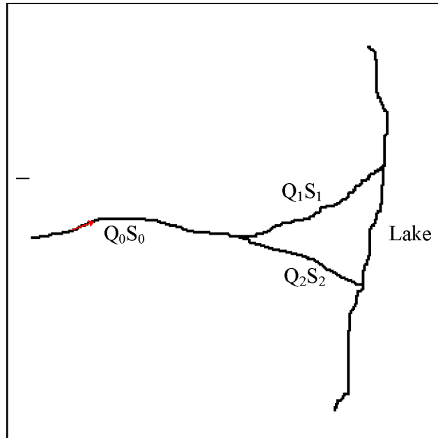
Fig.2 River bifurcation
