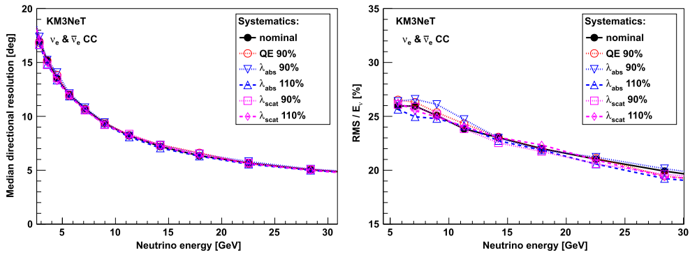
Figure 92. Resolution of the shower reconstruction for different water properties ( \lambda_{abs} and \lambda_{scat} ) and quantum efficiencies (QEs) for up-going \nu_e CC and \bar{\nu}_e CC events. Median neutrino direction (left) and relative energy resolution RMS/E_\nu (right).
