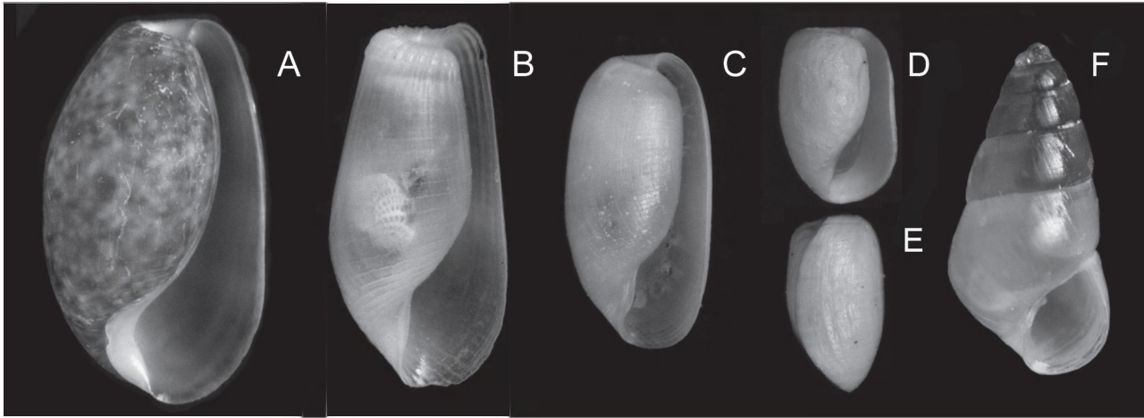
FIG. 4. – Opisthobranch and Pyramidellid gastropods of Zostera marina . A, apertural view of Bulla striata (Shell height: 12 mm); B, apertural view of Pyrrunculus hoernesii (2.2 mm), with a benthic foraminifer visible by transparency; C, apertural view of Cylichmina crosseii (1.8 mm); D, E, apertural and lateral view of Retusa minutissima (0.9 mm); F, apertural view of Odostomia turrata (1.7 mm).
