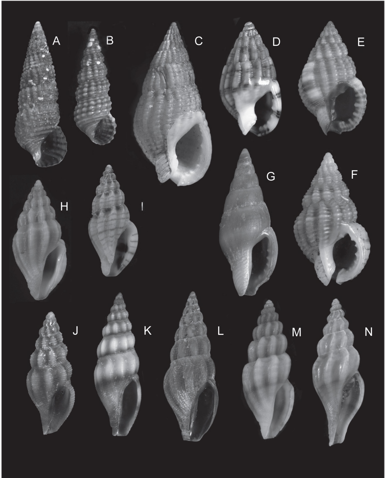
FIG. 3. – Prosobranch gastropods of the sediment and the leaf stratum in Zostera marina . Apertural views of: A, Bittium latreilli (Shell height: 7.4 mm); B, Bittium reticulatum (3.8 mm); C, Nassarius reticulatus (12.2 mm); D, Nassarius cuvierii (7.7 mm); E, Nassarius pygmaeus (8.7 mm); F, Nassarius incrassatus (10.2 mm); G, Mitrella minor (9.2 mm); H, Mangelia unifasciata (8.3 mm); I, Mangelia paciniana (6.1 mm); J, Bela sp. 1 (5.8 mm); K, Bela laevigata (9.9 mm); L, Bela nebula (8.5 mm); M, Bela costulata (7.7 mm); N, Mangelia attenuata (8.1 mm).
