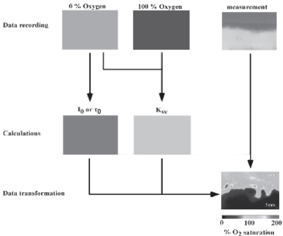
Figure 3. Knowing the \alpha -value, images of the two constants required by the modified Stern-Volmer equation ( I_0 (or \tau_0 ) and K_{sv} ) can be derived by a two-point calibration and measuring data can be transformed into O_2 images. The presented image was obtained at a diatom covered sediment and the horizontal heterogeneity is apparent, scale bars and sediment surface is included. For further discussion on the image please refer to Fenchel and Glud 2000.
