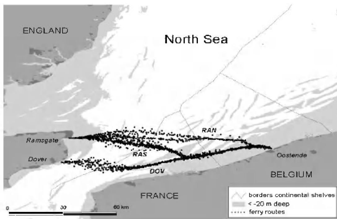
Fig. 1. The three routes followed by ferries during ship-based seabird surveys between Oostende and Dover/Ramsgate in 1992-98 (DOV=Dover route, RAN=northern route to Ramsgate, RAS=southern route to Ramsgate).
