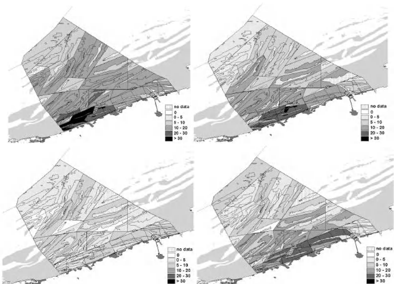
Fig. 16. The disturbance-sensitivity for seabirds in Belgian marine waters in: a) winter b) spring c) summer d) autumn. Shading is based on a disturbance sensitivity value, calculated from the relative abundance and the disturbance sensitivity of the 23 most abundant species.
