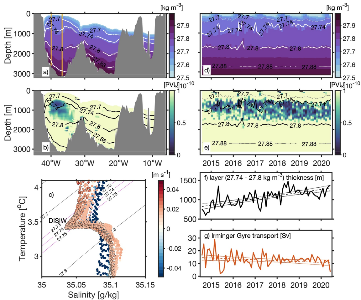
Figure 3. Mean (2014–2020) (a) density and (b) potential vorticity (PV) across the lower limb of Overturning in the Subpolar North Atlantic Programme (OSNAP) East, defined using the mean value of the isopycnal of maximum overturning, 27.57 \text{ kg m}^{-3} . (c) Conservative temperature and absolute salinity diagram of the time-averaged profiles at every longitude point between the East Greenland coast and the eastern limit of the Irminger Gyre (IG) (easternmost yellow line in panel (a)); profiles are colored by velocity ( \text{m s}^{-1} ) and data points outlined in black indicate profiles from IG region. The pink lines show the isopycnals that correspond to the Deep Irminger Sea Intermediate water (DISIW) in the region of interest. Temporal evolution of the (d) density and (e) PV in the zonally averaged IG region (yellow lines in panels (a, b)) indicating an increase in lower intermediate waters over time. Time series and trends of the DISIW layer ( 27.4\text{--}27.8 \text{ kg m}^{-3} ) (f) thickness and (g) IG transport over OSNAP period. Dotted lines in panels (f, g) indicate 95% confidence intervals.
