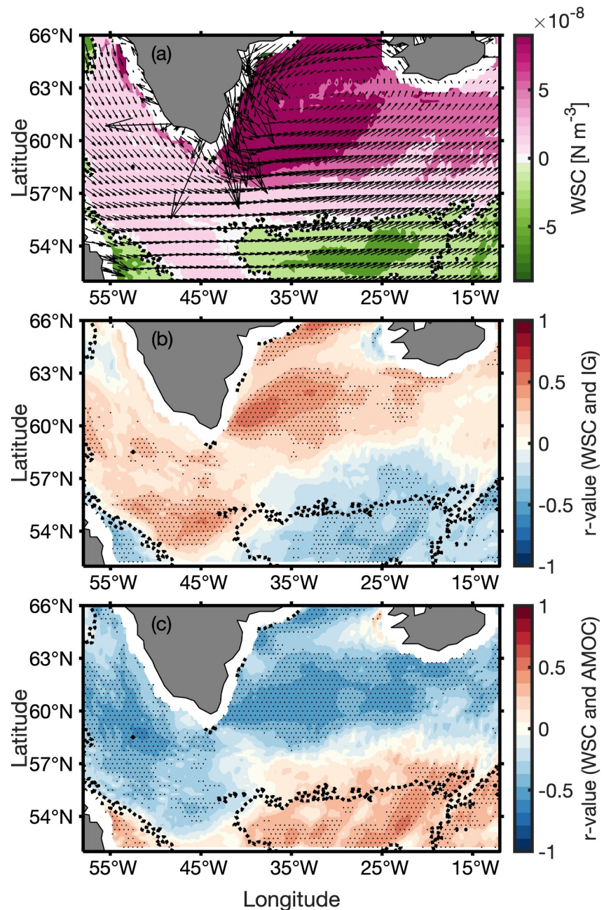
Figure 4. (a) Wind stress (vectors) and wind stress curl (WSC) (contours) over the 2014–2018 positive North Atlantic Oscillation period (December 2014–October 2018). Correlation between the WSC and the Irmingier Gyre transport at (b) the Overturning in the Subpolar North Atlantic Programme array and (c) the Atlantic meridional overturning circulation. Black dotted contour (a–c) indicates the zero WSC line. Stippling in panels (b, c) indicates statistical significance at 95% level.
