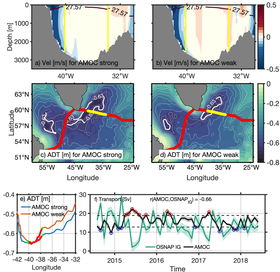
Figure 2. Composites of mean velocity in the interior Irminger Sea during (a) Atlantic meridional overturning circulation (AMOC) strong and (b) AMOC weak periods. (c, d) Same as in (a, b) but for absolute dynamic topography (ADT) over the subpolar North Atlantic. Red line in panels (c, d) indicates the location of Overturning in the Subpolar North Atlantic Programme (OSNAP) array, while yellow line indicates the span of the interior Irminger Sea, corresponding to yellow lines in panels (a, b). ADT contours are shown at 0.05 m intervals. (e) ADT over the Irminger Sea along OSNAP line for AMOC strong and weak periods. AMOC strong periods are defined as events one standard deviation above the mean AMOC value, and vice versa. (f) Volume transport of the Irminger Gyre (green line) compared with the AMOC from OSNAP East (black line). Red and black circles in panel (f) indicate AMOC strong and weak periods, respectively. Correlation is significant at 99% level. Shading indicates monthly uncertainty estimates using a Monte Carlo technique.
