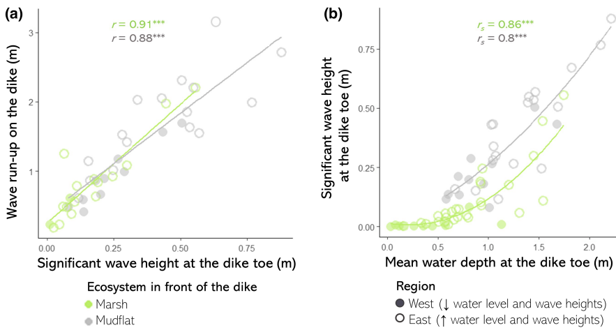
FIGURE 5 Relationships between (a) significant wave height and wave run-up on the dike, separated by salt marshes (green) and bare tidal flats (grey), excluding points with zero run-up, which occurred in cases where the waves were completely attenuated and (b) mean water depth and significant wave height including all the storm dates with wave run-up measured. Significant codes refer to p < 0.001 (***)
