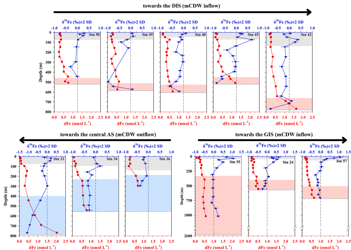
Fig. 4. Vertical water column profiles of dissolved Fe concentration ( [dFe] ) and \delta^{56}Fe from GPPr12 stations. [dFe] (red dots) corresponds to the bottom x-axis; whereas \delta^{56}Fe (blue dots) corresponds to the top x-axis (error bar show two standard deviation (SD) for most samples, for samples that have 2 standard error lower than the long-term 2 SD of the internal standard – NIST SRM 3126a ( +0.36 \pm 0.05 \% , n = 524 ), 0.05 is assigned as 2 SD). The grey dashed line indicates 0 ‰ of \delta^{56}Fe , whereas the black dotted line indicates the bottom depth. The grey shading marks the surface layer (surface to fluorescence maximum depth); whereas the red and blue bars mark the depth of the mCDW inflow and outflow, respectively.
