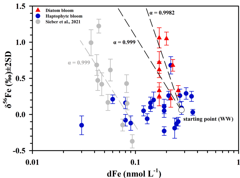
Fig. 7. Fe isotope systematics in the surface layer of the GPp12 ‘bloom’ stations (red: GIS diatom bloom; blue: DIS haptophyte bloom), in comparison with data derived from Mertz glacier polynya (Sieber et al., 2021). The dashed lines represent predicted Rayleigh fractionation trends with different fractionation factors ( \alpha = R_{\text{biomass}}/R_{\text{seawater}} ) based on a defined starting point (empty white dot, observed [dFe] and \delta^{56}\text{Fe} values in winter water).
