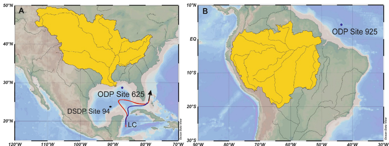
Fig. 1. Locations of: (A) ODP Site 625 and DSDP Site 94 in the Gulf of Mexico, and (B) ODP Site 925 on the Ceara Rise. The modern watersheds of the (A) Mississippi and (B) Amazon Rivers are shaded in yellow. The position of the Loop Current (LC) in the Gulf of Mexico during austral summer (red) and fall/winter (blue) is shown. (For interpretation of the references to colour in this figure legend, the reader is referred to the web version of this article.)
