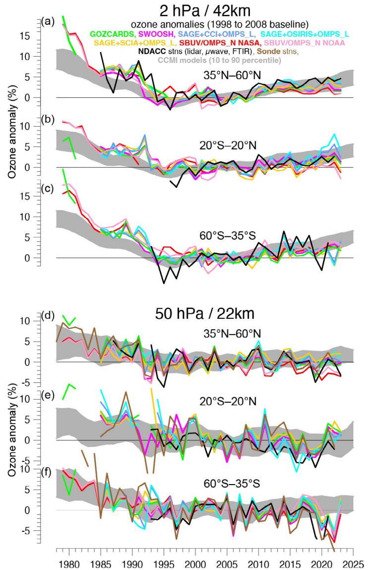
Fig. 2.72. Annual mean anomalies of ozone (%) in (a)–(c) the upper stratosphere near 42-km altitude or 2-hPa pressure, and (d)–(f) the lower stratosphere, near 22 km or 50 hPa for three zonal bands: 35°N–60°N, 20°S–20°N (tropics), and 35°S–60°S, respectively. Anomalies are with respect to the 1998–2008 baseline. Colored lines are long-term records obtained by merging different limb (GOZCARDS, SWOOSH, SAGE+CCI+OMPS_L, SAGE+OSIRIS+OMPS_L, SAGE+SCIAMACHY+OMPS_L) or nadir-viewing (SBUV, OMPS_N) satellite instruments. The nadir-viewing instruments have much coarser altitude resolution than the limb-viewing instruments. This can cause differences in some years, especially at 50 hPa. The black line is determined from merging ground-based ozone records at seven Network for the Detection of Atmospheric Composition Change (NDACC) stations employing differential absorption lidars and microwave radiometers. See Steinbrecht et al. (2017), Arosio et al. (2019), and Godin-Beekmann (2022) for details on the various datasets. Gray-shaded areas show the range of chemistry-climate model simulations from CCM1 refC2 (SPARC/IO3C/GAW 2019). Ozone data for 2023 are not yet complete for all instruments and are still preliminary.
