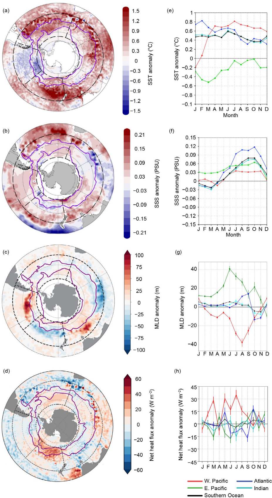
Fig. 6.13. Annual-average anomalies (Jan–Dec 2023) of (a) sea-surface temperature (SST; °C), (b) sea-surface salinity (SSS; PSU), (c) mixed-layer depth (MLD; m), and (d) net heat flux ( W m^{-2} ). Overlaid are the positions of the Subantarctic and Southern Boundary Antarctic Circumpolar Fronts (purple lines) as defined by Orsi et al. (1995). Four distinct regions between 40°S and 65°S are delineated by black dashed contours corresponding to the Atlantic (70°W–20°E), Indian (20°E–170°E), western Pacific (170°W–120°W), and eastern Pacific (120°W–70°W) sectors. The 2023 seasonal cycle of anomalies in (e) SST (°C), (f) SSS (PSU), (g) MLD (m), and (h) net heat flux ( W m^{-2} ) separated according to the four sectors defined above. Error bars in (g),(h) represent the standard error of the climatological mean (i.e., std. dev. divided by \sqrt{N} , where N is the number of years, the number of years in the climatology).
