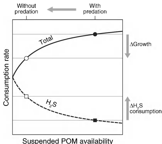
FIG. 6. Schematic depiction of a possible mechanism showing how Loripes may experience growth in the absence of predation on Dosinia . Without predation, Dosinia densities will be higher, and hence suspended POM (particulate organic matter) availability will be lower. Assuming that in Loripes the consumption of suspended POM is mutually exclusive with the utilization of sulfide, the absolute use of sulfide will increase when suspended POM availability decreases, although the total consumption rate (suspended POM and sulfide), and hence the growth rate, will decline.
