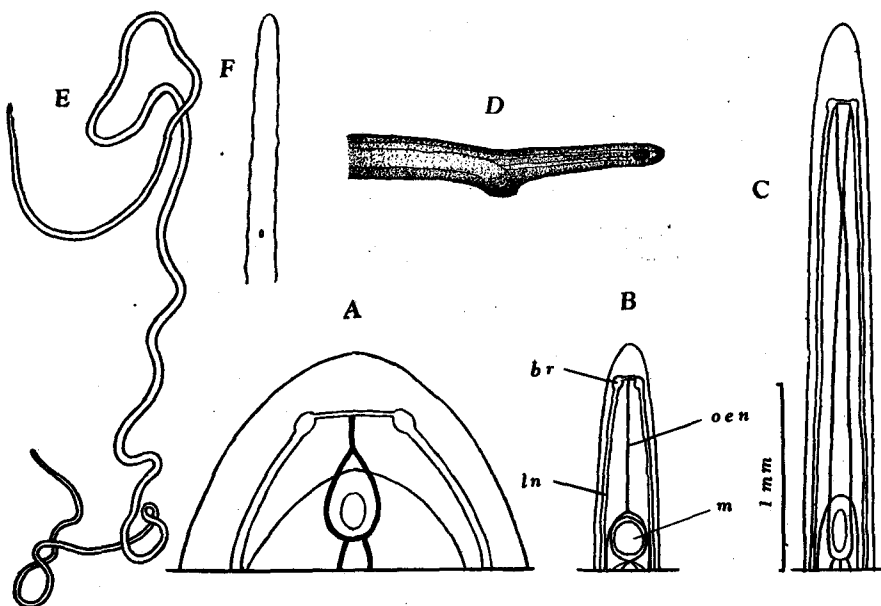
Fig. 1. A-C. Diagram of organs in the anterior portion of the body showing the nervous system in three species (A. Procephalothrix simulus Iwata B. P. filiformis (Johnston), C. Cephalothrix notabilis nov. sp.). D. P. filiformis . Lateral surface in the anterior portion of the body. E. C. notabilis . Dorsal surface of the body. F. C. notabilis . Ventral surface of the body. For abbreviation, see p. 39.
