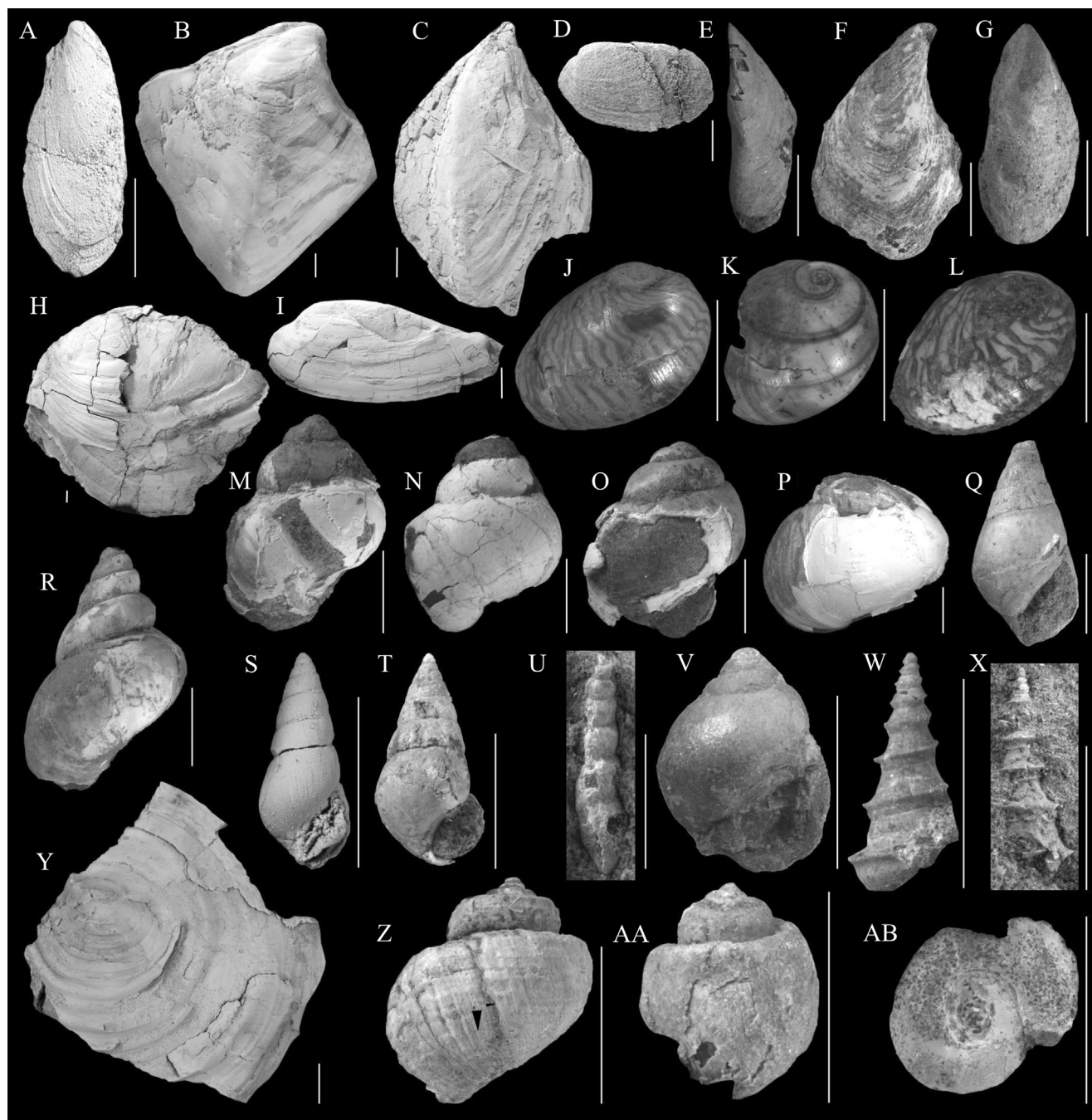
Fig. 6. Bivalve (dreissenids and unionids) and gastropod species from the study section with indicated sample number. A. Coelogonia pseudorostriformis (Sinzov, 1897), ME13/22. B. Congerina ( Rhombocongerina ) rhomboidea Hoernes, 1867, ME13/26. C. Congerina ( Rhombocongerina ) unica Papaianopol and Macalet, 1998, ME13/26. D. Dreissenomya rumana (Wenz, 1942), ME13/21. E. Dreissena tenuissima Sinzov, 1875, ME13/31a. F. Dreissena ( Pontodreissena ) rostriformis corniculata Stefanescu, 1896, ME16/63. G. Dreissena ( Modiolodreissena ) rimestiensis Fontannes, 1887, ME13/28. H. Hyriopsis krausi (Wenz, 1932), ME13/31a. I. Rumanunio rumana (Tournouër, 1879), ME13/31a. J. Theodoxus galeatus (Marinescu, 1962), ME16/74. K. Theodoxus quadrifasciatus (Bielz, 1864), ME13/36. L. Theodoxus scriptus (Stefanescu, 1896), ME13/30. M. Viviparus achatinoides (Deshayes, 1838), ME16/73. N. Viviparus botenicus Lubenescu and Zazuleac, 1985, ME13/32. O. Viviparus wesselinghi Neubauer, Harzhauser, Georgopoulou, Mandic and Kroh, 2014, ME13/37. P. Viviparus cf. papaianopoli Lubenescu and Zazuleac, 1985, ME13/40. Q. Melanopsis decollata Stoliczka, 1862, ME16/71. R. Tylopoma speciosa (Cobălcescu, 1883), ME16/63. S. Hydrobia pontilitoris Wenz, 1942, ME13/33. T. Hydrobia spicula Stefanescu, 1896, ME16/73. U. Prososthenia cf. radmanesti (Fuchs, 1870), ME16/66. V. Lithoglyphus rumanus Stefanescu, 1896, ME13/31a. W. Pyrgula botenensis Wenz, 1942, ME13/37. X. Pyrgula cf. atava Brusina, 1881, ME16/97. Y. Valenciennius annulatus Rousseau, 1842, ME16/80. Z. Zagrabica carinata Andrusov, 1909, ME16/79. AA. Zagrabica reticulata Stefanescu, 1896, ME16/75. AB. Gyraulus rumanus Wenz in Krejci-Graf and Wenz, 1932, ME16/96. Scale bars: 5 mm.
