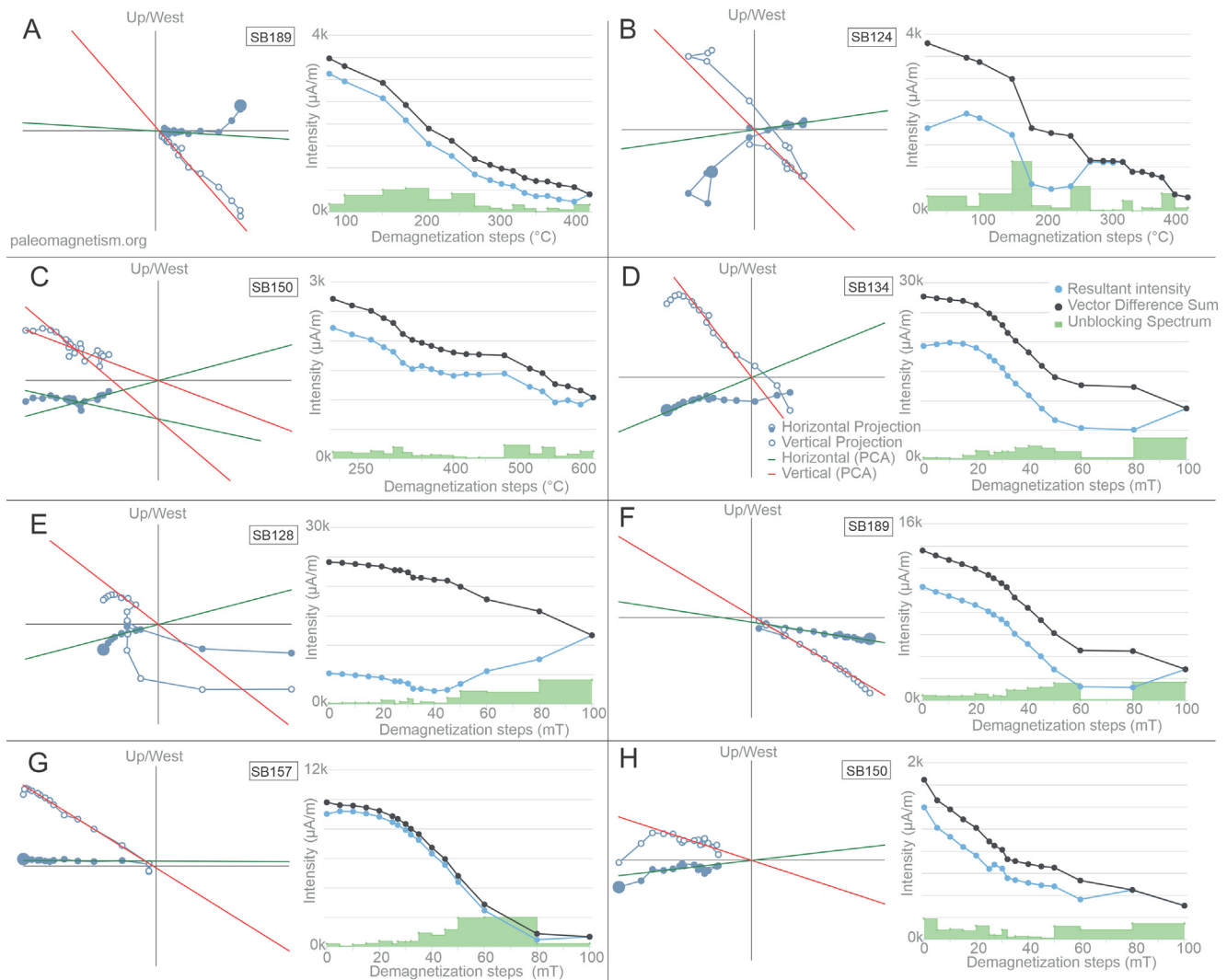
Fig. 4. Zijderveld diagrams and intensity diagrams for representative samples from the Pontian of Slănicul de Buzău. All Zijderveld diagrams are in tectonic coordinates. Figures made with paleomagnetism.org .
