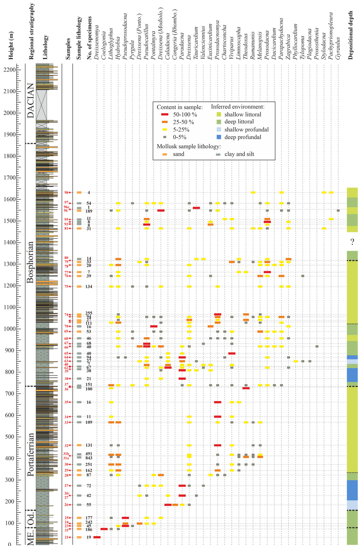
Fig. 7. Position of mollusk samples in the section with indicated lithology, their genus-level content with plotted abundances, and the resulting paleodepth interpretation (see text for details).
