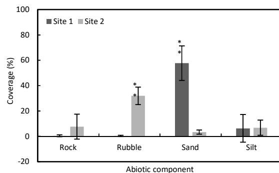
Figure 6. The study sites cover Abiotic components in the coral reef ecosystems. Information: ** is significantly different (T-independent test, P < 0.05 ).
