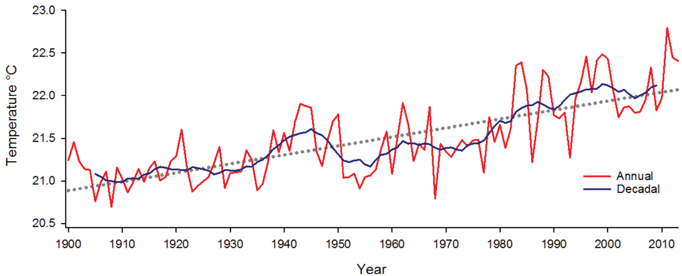
Figure 3. The annual mean surface temperatures (red line) at the Houtman Abrolhos Islands ( 28^{\circ} – 29^{\circ} S) off the midwest coast of Western Australia between 1900 and 2013, from the HadISST data set ( http://apdrc.soest.hawaii.edu/datadoc/hadisst1.php ), and the 11-year moving average to approximate decadal variability (blue line). The straight dotted line is the linear trend for the individual annual mean temperatures. The mean temperature rise was about 0.1^{\circ}\text{C} per decade.
