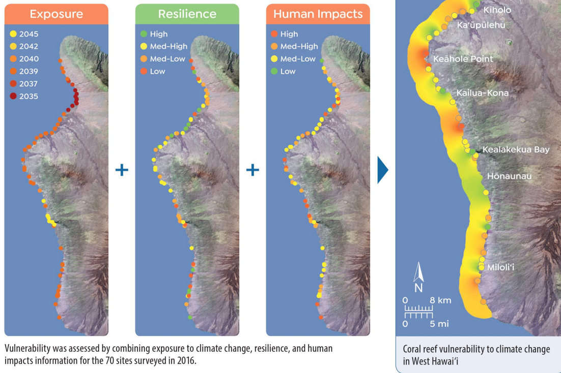
Figure 8. Example of climate vulnerability assessment from West Hawai'i (see hyperlink for full report - NOAA et al. 2019 ) showing result of combing climate model projections of bleaching conditions with data on relative resilience and human impacts.
