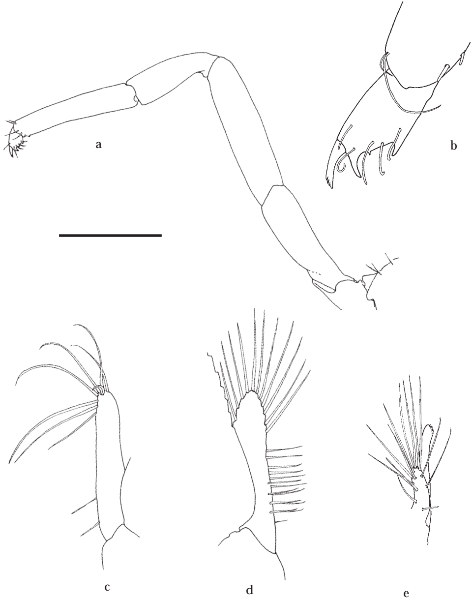
Fig. 245. Odontonia sibogae (Bruce, 1972): ovigerous female, pochl. 5.2 mm (fig. c); male, pochl. 5.0 mm (figs. a, d, e), RMNH D 46697; non-ovigerous female, pochl. 1.6 mm (fig. b). a, third pereiopod; b, dactylus third pereiopod; c, endopod female first pleopod; d, endopod male first pleopod; e, appendix interna and appendix masculina on second male pleopod. Scale: a = 1.5 mm; b = 0.15 mm; c-e = 0.6 mm.
