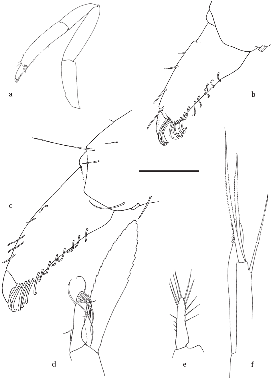
Fig. 240. Odontonia seychellensis spec. nov.: male holotype, pochl. 2.6 mm (figs. c, e, f), non-ovigerous female paratype, pochl. 3.5 mm (figs. a, b, d), RMNH D 42558. a, third pereopod; b, dactylus third pereopod male; c, dactylus third pereopod female; d, endopod female first pleopod; e, endopod male first pleopod; f, appendix interna and appendix masculina on second male pleopod. Scale: a = 1.5 mm; b, c, f = 0.15 mm; d, e = 0.6 mm.
