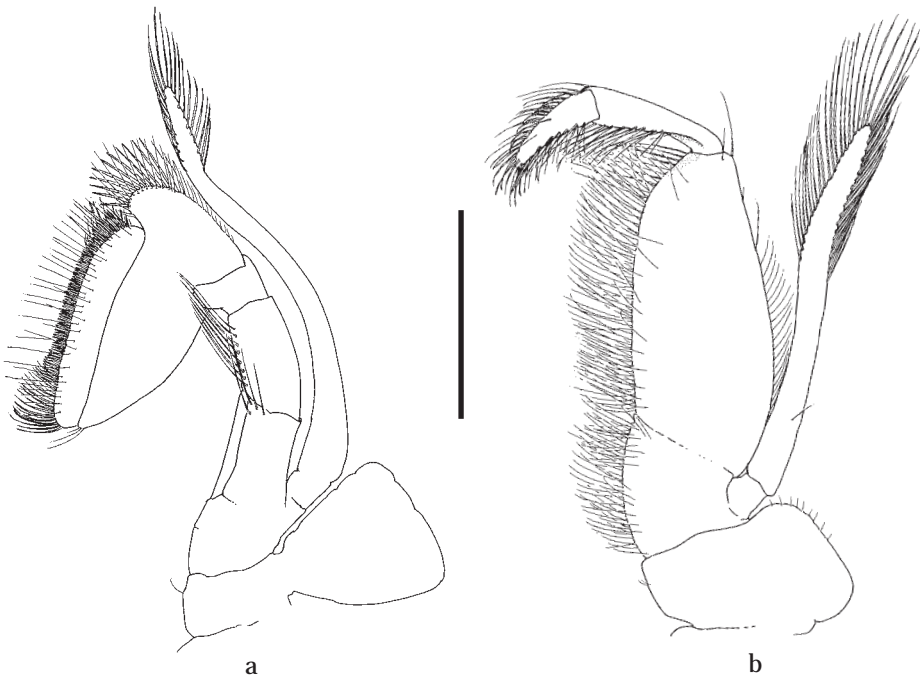
Fig. 85. Pontonia mexicana Guérin, 1856: ovigerous female, pocl. 8.6 mm, RMNH D 42641. a, second maxilliped, ventral view; b, third maxilliped, ventral view. Scale = 1.9 mm.
