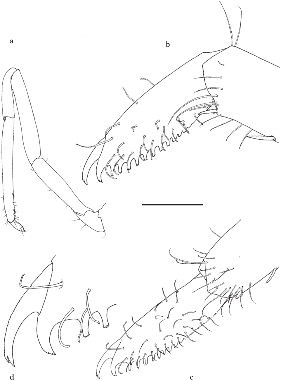
Fig. 191. Dactyлонia ascidicola (Borradaile, 1898): 1 male, pochl. 3.3 mm (fig. b), RMNH D 42562; 1 male, pochl. 3.3 mm (fig. a), RMNH D 46789; ovigerous female, pochl. 2.5 mm, RMNH D 42565 (figs. c, d). a, third pereopod; b, dactylus third pereopod; c, idem; d, idem, detail unguis. Scale: a = 1.5 mm; b, c = 0.15 mm; d = 0.06 mm.
