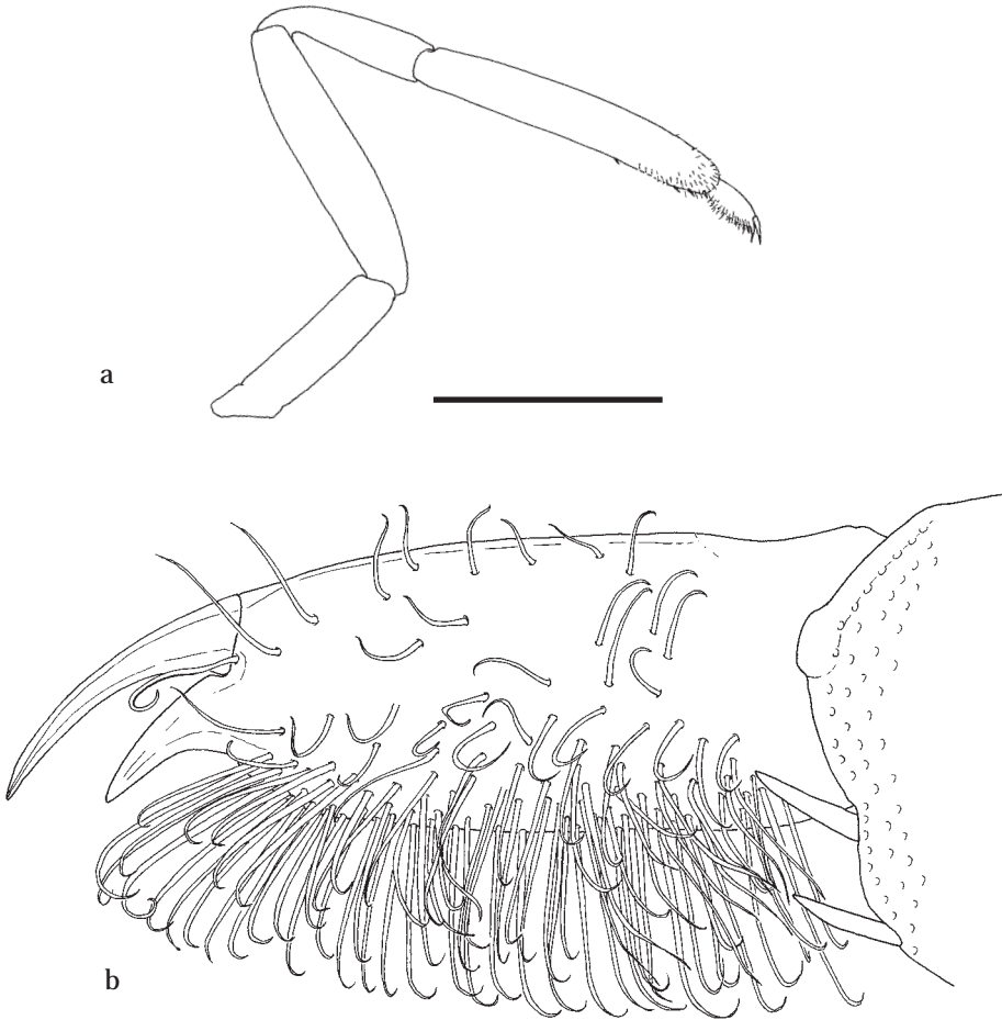
Fig. 145. Ascidonia flavomaculata (Heller, 1864): ovigerous female, pochl. 4.8 mm, RMNH D 45616. a, third pereiopod; b, dactylus third pereiopod. Scale: a = 2 mm; b = 0.15 mm.
