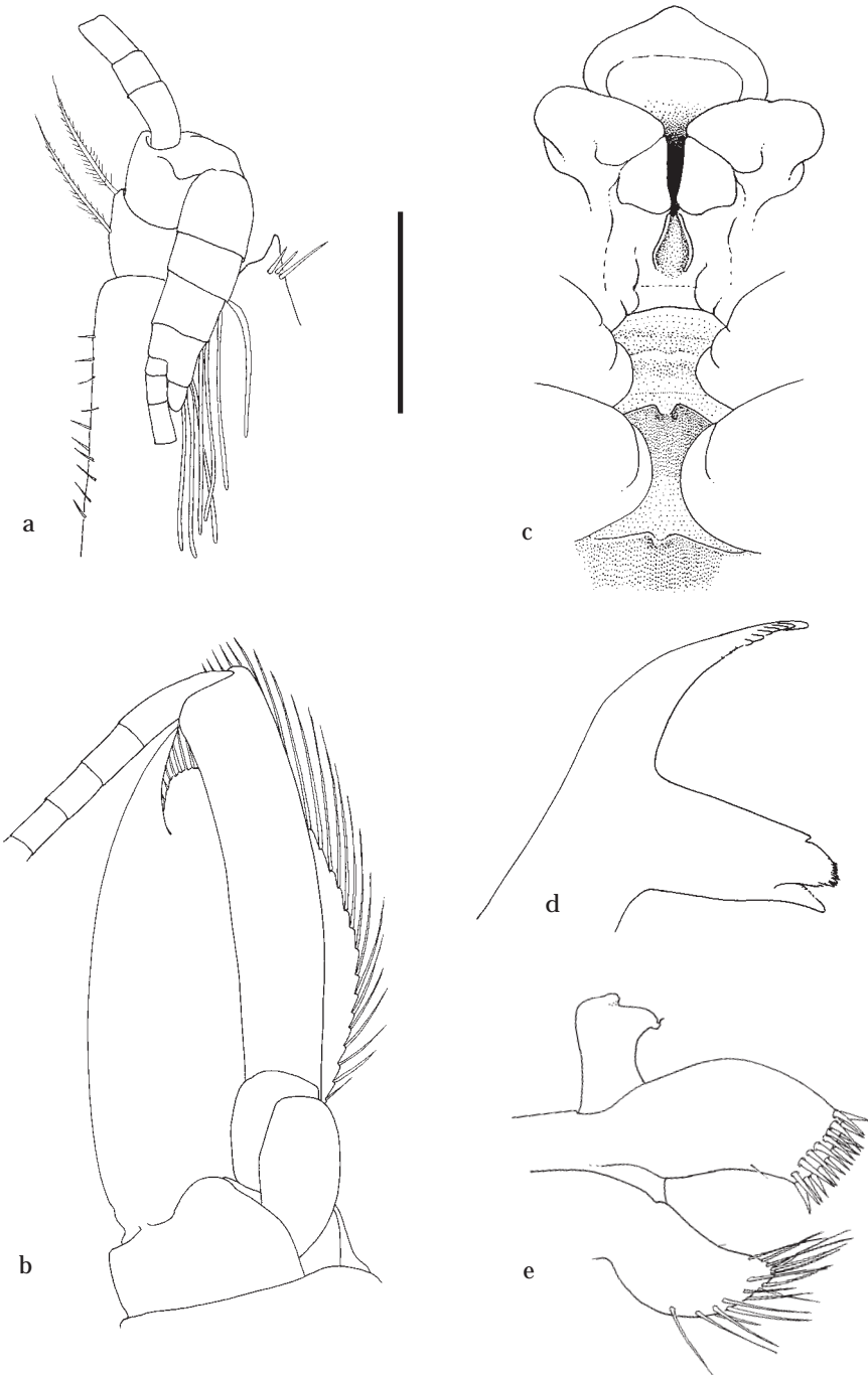
Fig. 231. Odontonia rufopunctata spec. nov.: ovigerous female holotype, pochl. 4.0 mm, RMNH D 46702. a, antennula, dorsal aspect of distal part; b, antenna, ventral view; c, paragnath and second to fifth thoracic sternites; d, mandible, ventral view; e, maxillula, ventral view. Scale: a, b, d, e = 0.6 mm; c = 1 mm.
