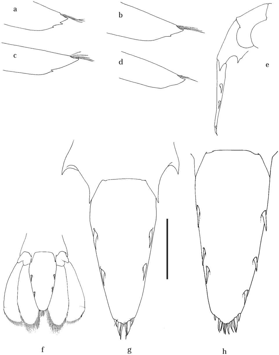
Fig. 112. Pontonia pinnophylax (Otto, 1821): ovigerous female, pochl. 10.4 mm (fig. a), male, pochl. 10.6 mm (fig. b), male, pochl. 9.4 mm (fig. c), RMNH D 26479; ovigerous female, pochl. 10.5 mm (fig. d), RMNH D 26985; male, pochl. 6.6 mm (figs. e, g), ovigerous female, pochl. 6.9 mm (fig. f), RMNH D 15167; USNM 273526 (fig. h). a-d, distal tip of rostrum, lateral view; e, distal part abdomen, lateral view; f, telson and uropods, dorsal view; g, h, telson, dorsal view. Scale: a-d = 1 mm; e, f = 4 mm; g, h = 2 mm.
