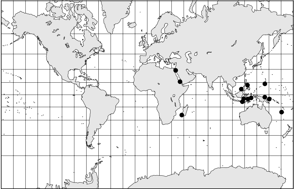
Fig. 193. Geographic distribution of Dactyлонia ascidicola (Borradaile, 1898).
