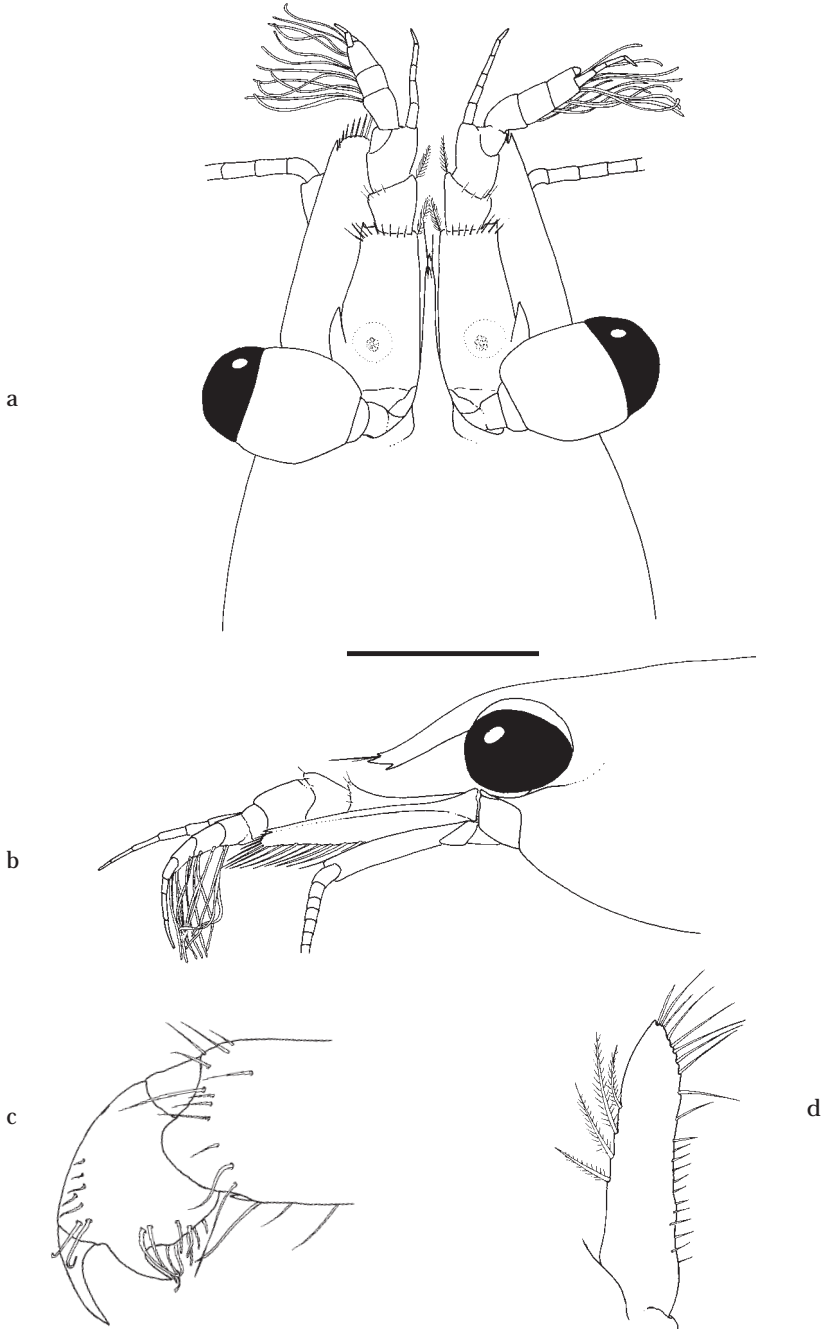
Fig. 69. Pontonia manningi Fransen, 2000: Cape Verde Islands, juvenile, pochl. 1.9 mm, RMNH D 45624 (figs. a-c ); male, pochl. 4.8 mm, RMNH D 48667 (fig. d). a, anterior appendages, dorsal view; b, anterior appendages, lateral view; c, dactylus third pereiopod; d, male first pleopod. Scale: a, b = 1 mm; c = 0.15 mm; d = 0.6 mm.
