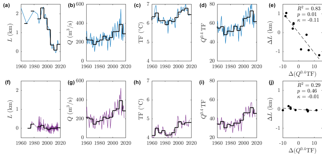
Figure 4. Example calibration of the retreat parameterization for two glaciers: Kangiata Nunata Sermia in southwestern Greenland (top row) and Store glacier in central western Greenland (bottom row). (a, f) Terminus position, (b, g) summer subglacial discharge, (c, h) ocean thermal forcing and (d, i) parameterized submarine melting. Light lines show all values in the datasets, while the heavy black lines show 5-year binning. (e, j) The 5-year binned values of parameterized submarine melt anomaly ( x axis) versus terminus position anomaly ( y axis). The text in (e) and (j) shows the correlation coefficient ( R^2 ), the significance of the regression ( p ) and the linear coefficient ( \kappa ).
