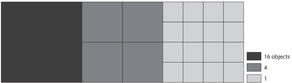
Figure 2. Only standardised data (rates etc.) should be mapped with choropleth maps. Inspired by Slocum (2009).
