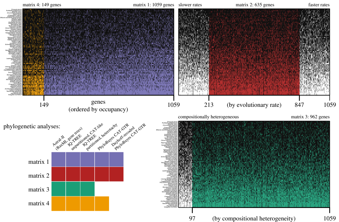
Figure 1. Matrices and phylogenetic methods used to infer gastropod relationships. With 50% taxon occupancy, matrix 1 is the largest, with 1059 genes. Matrix 4 is the subset of the best sampled 149 genes, with 70% taxon occupancy. Genes and species are sorted with the best sampling on the upper left. Matrix 2 is the subset of 635 genes after ordering all genes by evolutionary rate and removing the 20% slowest and 20% fastest evolving genes. Matrix 3 includes the 962 genes that are homogeneous in amino acid composition; genes are ordered by p -value of the homogeneity test. Black cells indicate genes present for each species. See Methods for details. (Online version in colour.)
