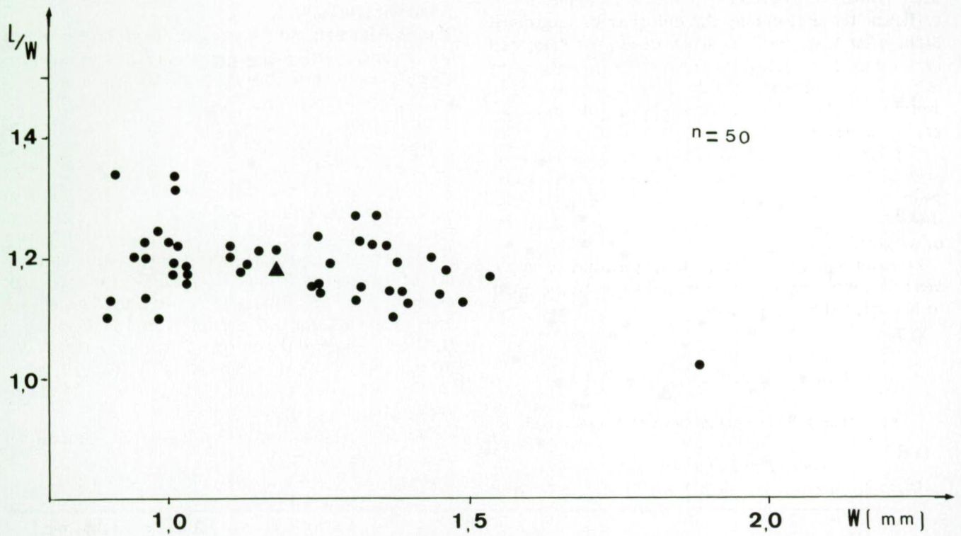
Fig. 4 — Scatter diagram of Argyrotheca popielae n. sp., Lower Maastrichtian. Ciplý. Ratio shell length (L in mm) to width (W in mm). ▲: holotype. Sample n°4.
