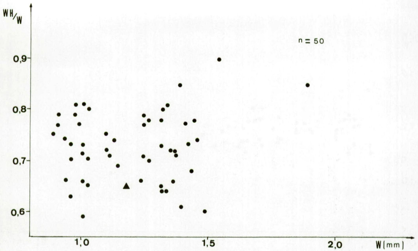
Fig. 6 — Scatter diagram of Argyrotheca popielae n. sp., Lower Maastrichtian. Cipl. Ratio hinge line width (WH in mm) to width (W in mm). ▲: holotype. Sample n° 4.
