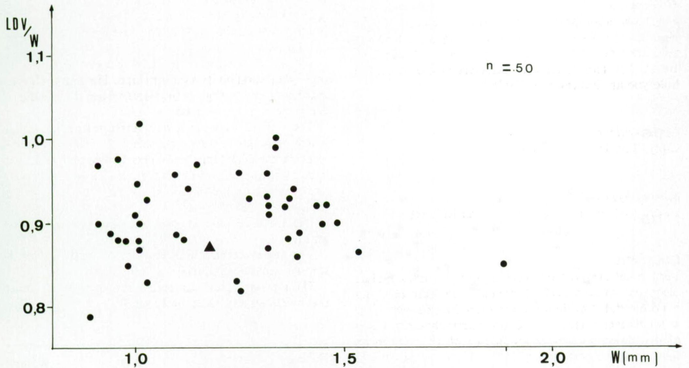
Fig. 5 — Scatter diagram of Argyrotheca popielae n. sp., Lower Maastrichtian. Ciplý. Ratio dorsal valve length (LDV in mm) to width (W in mm). ▲: holotype. Sample n°4.
