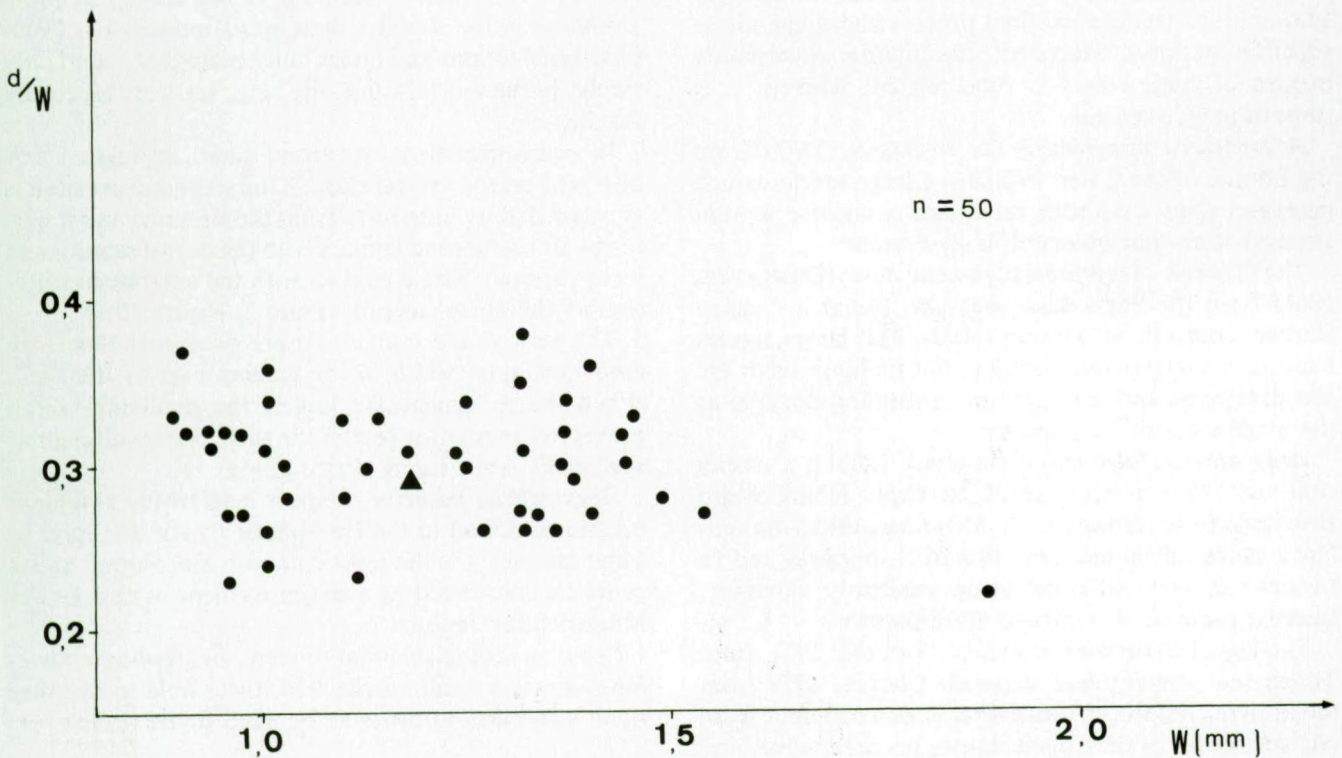
Fig. 8 — Scatter diagram of Argyrotheca popielae n. sp., Lower Maastrichtian. Ciplý. Ratio foramen diameter ( d/W in mm) to width ( W in mm). ▲: holotype. Sample n°4.
