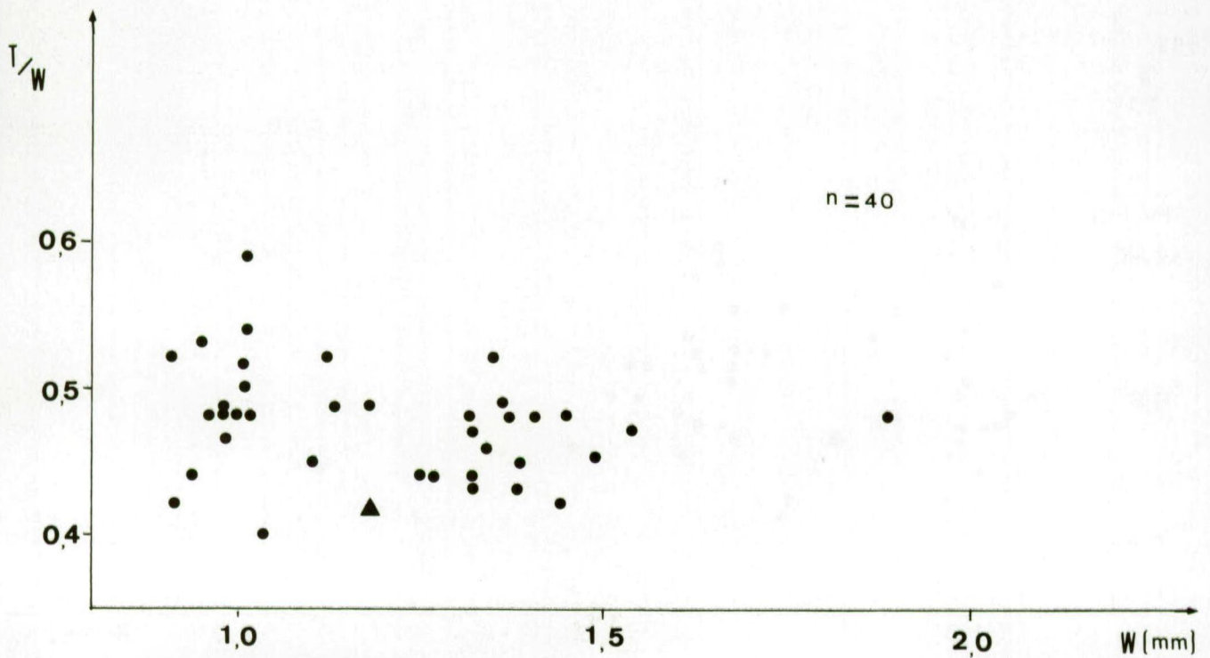
Fig. 7 — Scatter diagram of Argyrotheca popielae n. sp., Lower Maastrichtian. Cipl. Ratio thickness (T in mm) to width (W in mm). ▲: holotype. Sample n° 4.
