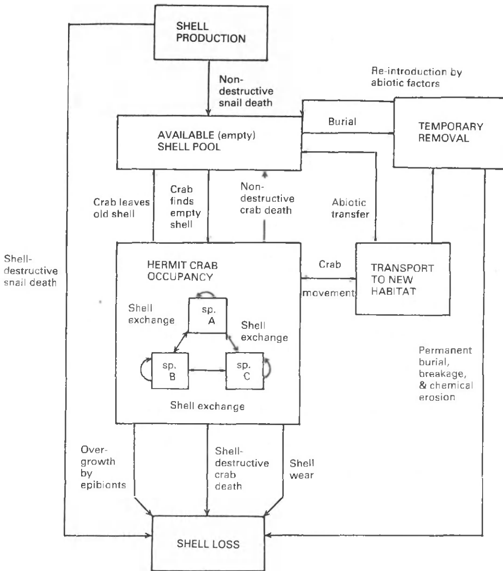
FIG. 7. Flowchart of shell movement in a guild of hermit crabs (after Hazlett, 1981a).
