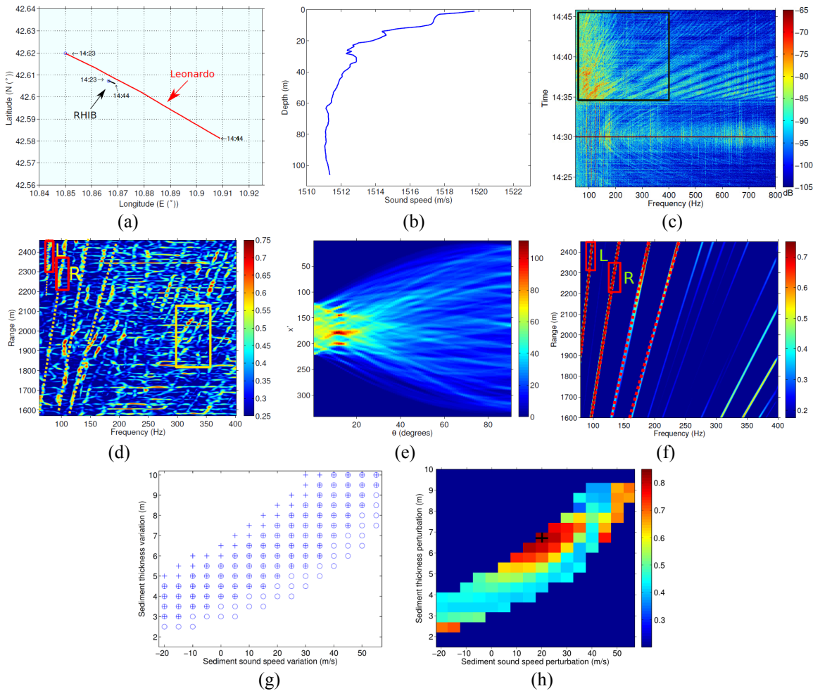
Figure 3. (a) Geometry of MREA/BP07 run L2, 23 April 2007. (b) Sound speed profiles (SSP) taken at R/V Leonardo just before the run. (c) The acoustic pressure spectrogram measured by a single hydrophone. (d) The calculated line structure of the boxed area in Fig. (c). (e) The Radon transform result of the yellow box area in Fig. (d). (f) The interference structure for reference sediment for a 19.6 m depth receiver and corresponding selected striations. (g) The estimations of the perturbations of sediment layer thickness and sound speed for the striations in (d) ('cross' is the results from striation L and 'circle' is the result from striation R). (h) The correlation coefficients between the Radon transform of data and that of possible values.
