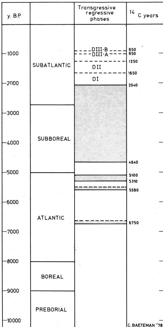
Fig. 2. - Chronological timescale.
