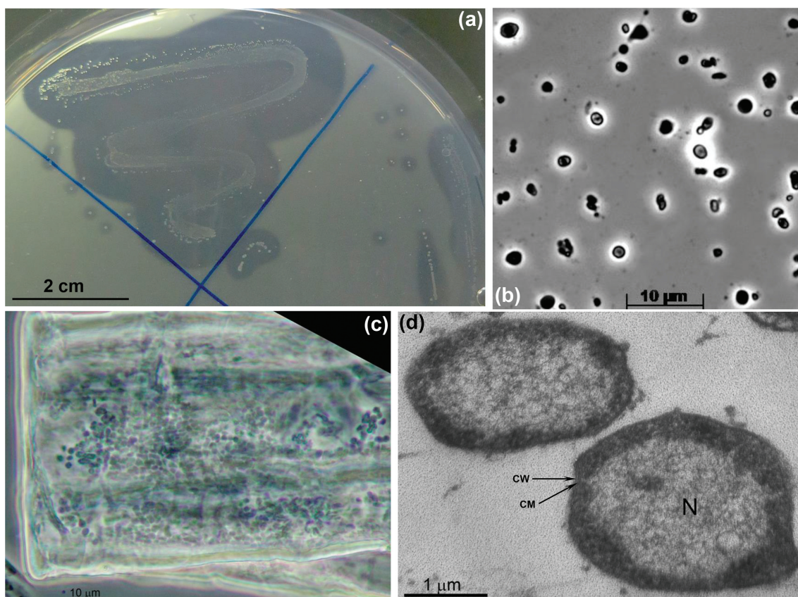
Fig. 1. Morphology of strain HArce11 T growing at 4 M total NaCl and 37 °C. (a) Colonies on amorphous cellulose plates forming large hydrolysis zones; (b) phase contrast microphotograph of cells grown with amorphous cellulose in liquid culture; (c) phase contrast microphotograph of cells forming biofilm on a cellulose fibre; (d) electron microscopy of thin sections of cells grown with amorphous cellulose. CW, cell wall; CM, cytoplasmic membrane; N, nucleoid.
